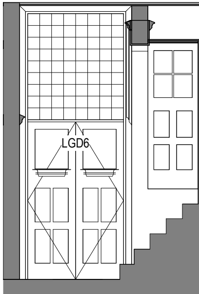
B0022 - Proposed Elevation B 1 : 50
