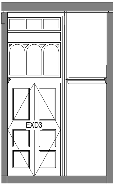
B0024 - Proposed Elevation B 1 : 50
