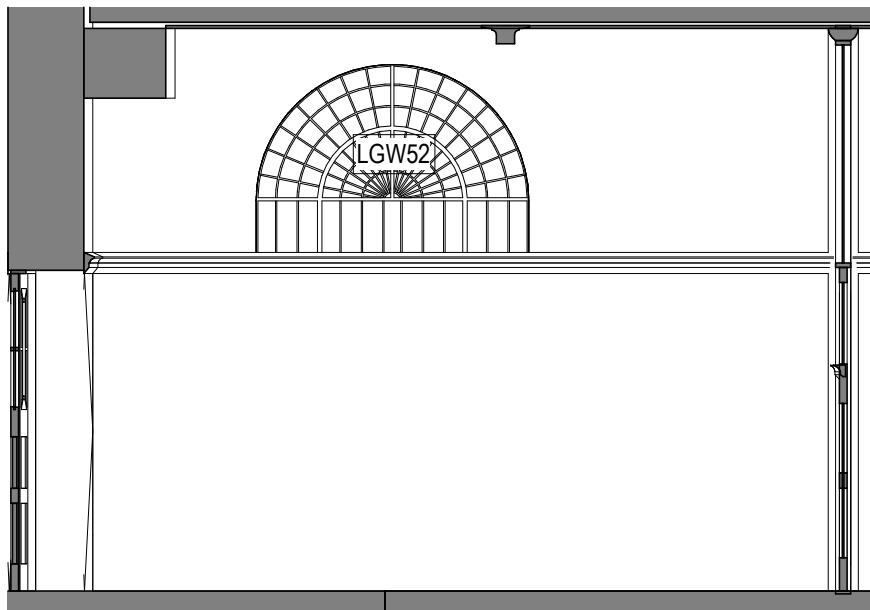
B0022 - Proposed Elevation A 1 : 50
