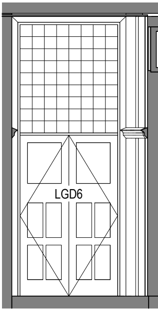
B0024 - Proposed Elevation D 1 : 50
