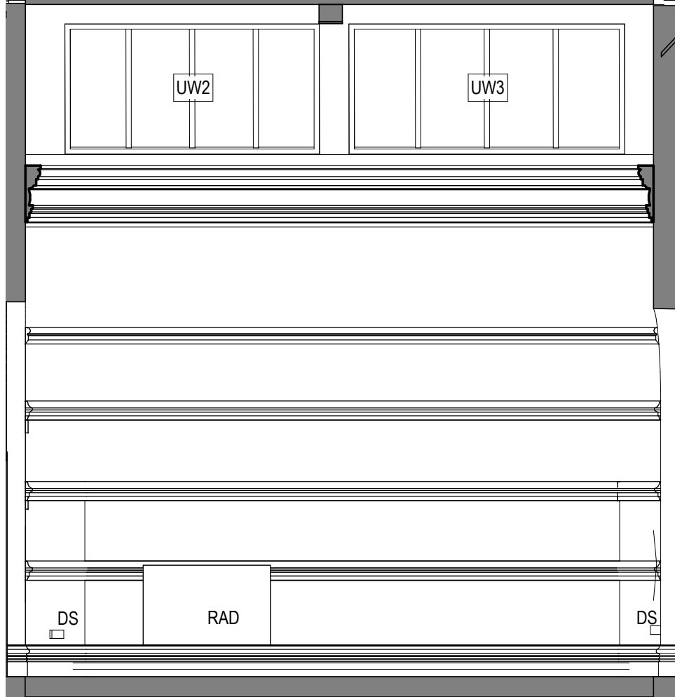
F0012 - Elevation A 1 : 50
