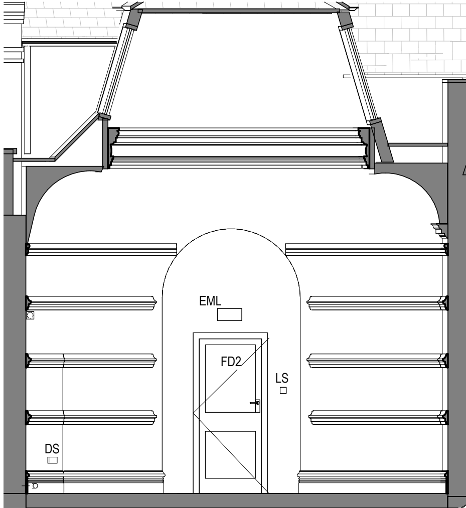
F0012 - Elevation B 1 : 50
