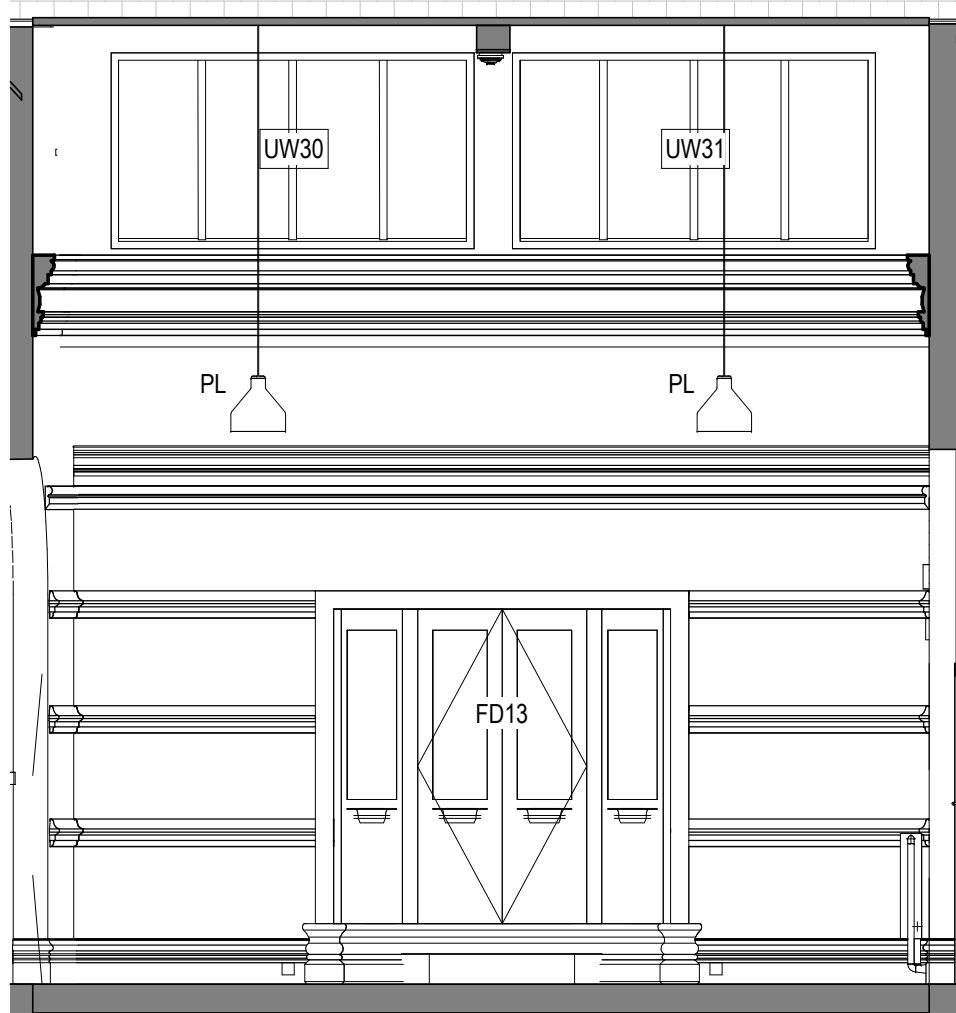
F0012 - Elevation C 1 : 50
