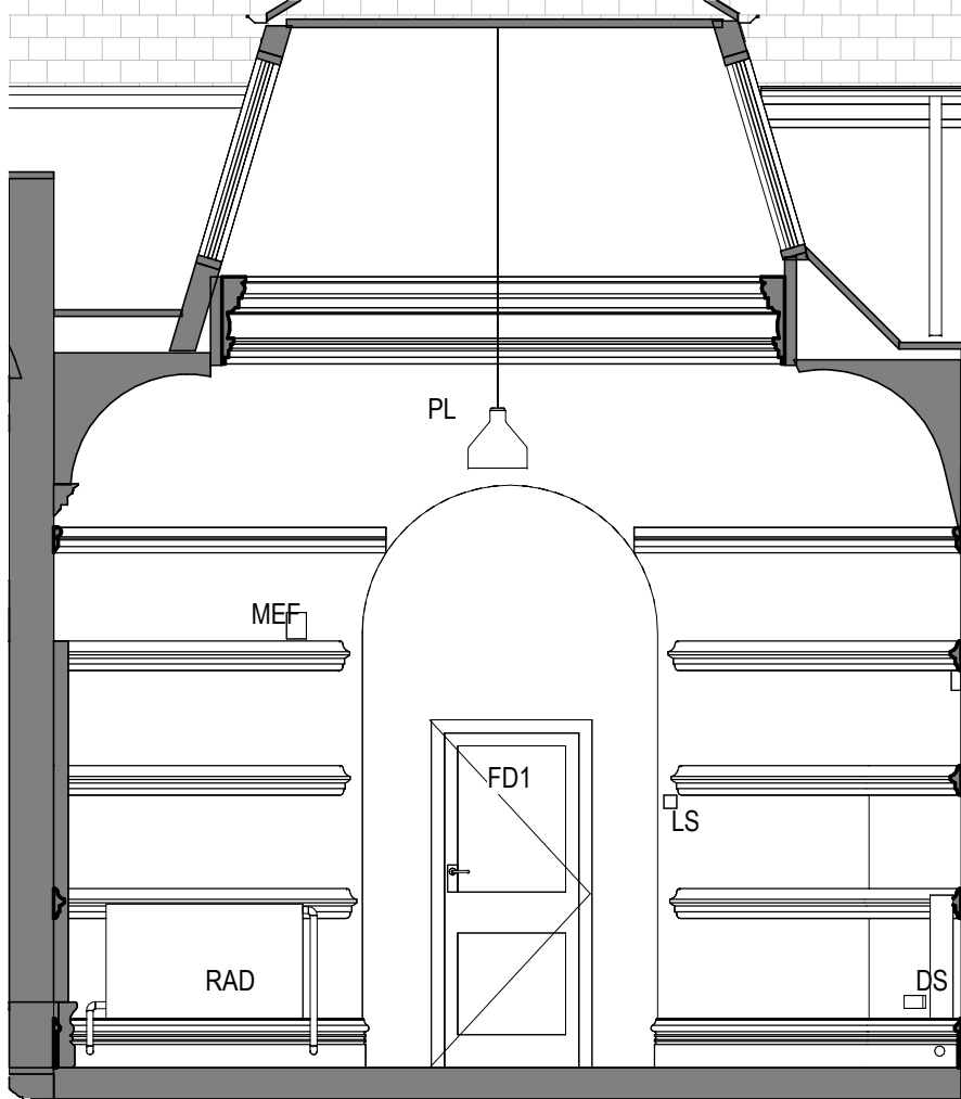
F0012 - Elevation D 1 : 50
