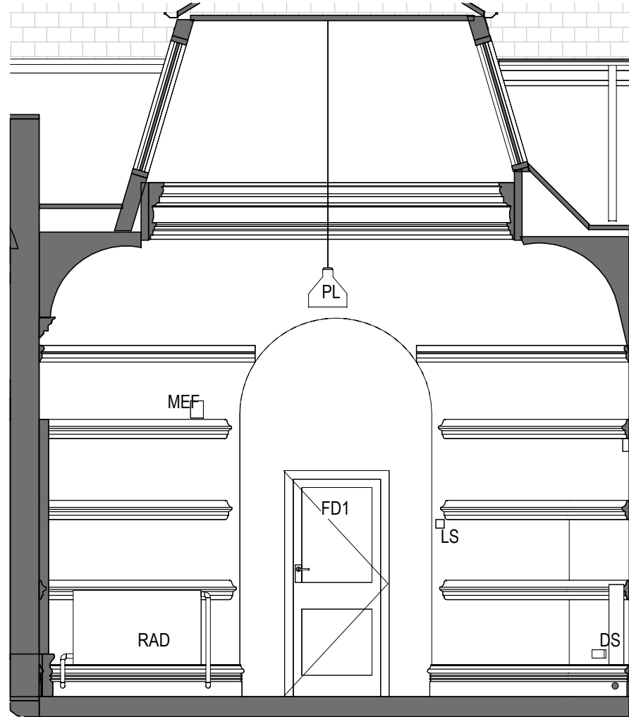
F0012 - Demolition Elevation D 1 : 50
