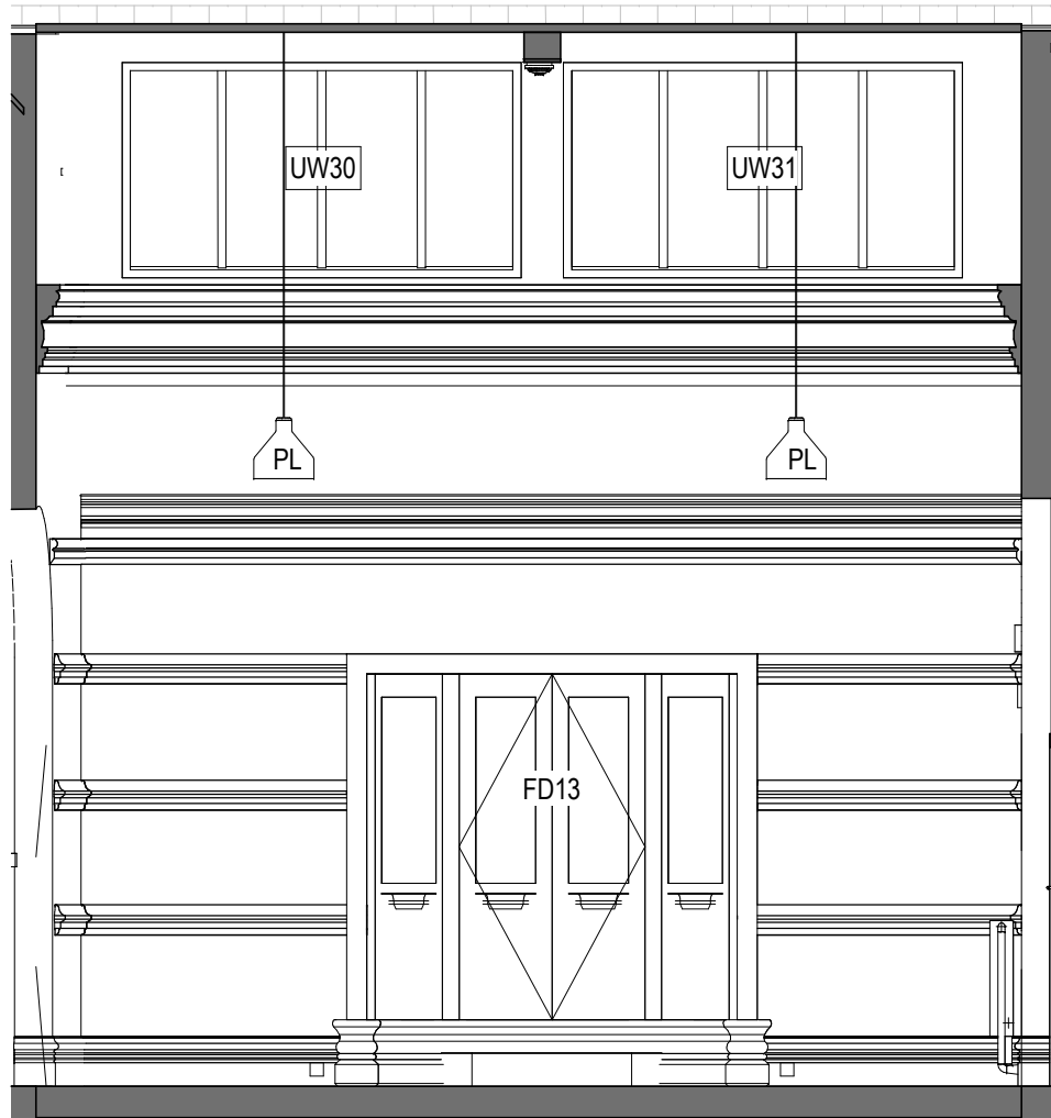
F0012 - Demolition Elevation C 1 : 50
