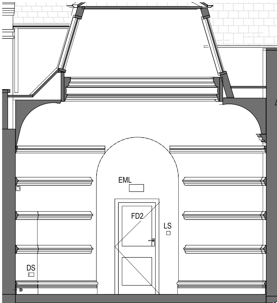
F0012 - Demolition Elevation B 1 : 50
