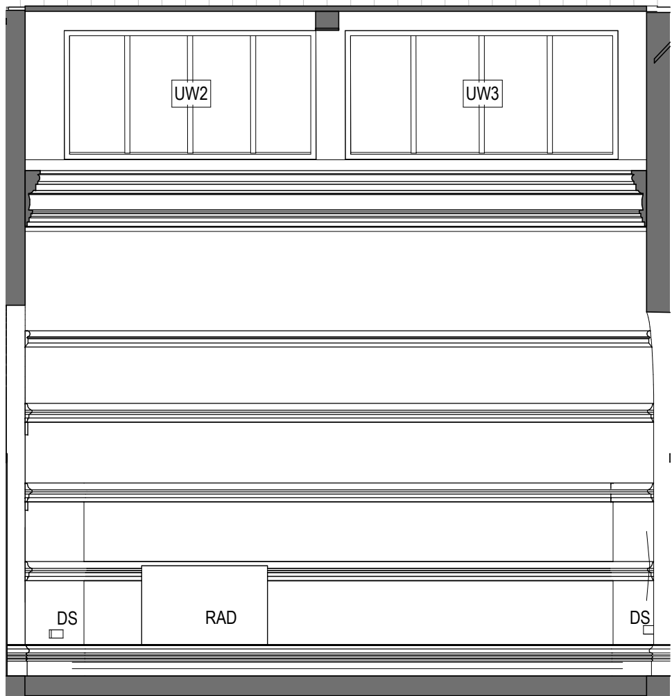
F0012 - Demolition Elevation A 1 : 50
