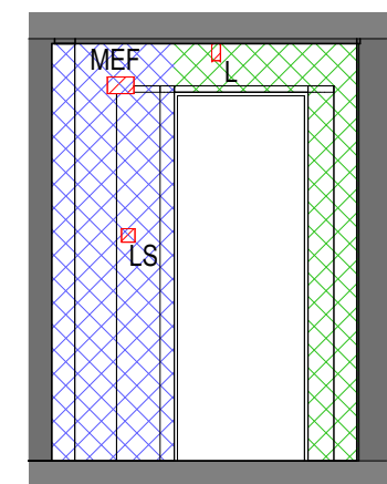
B0015 - Demolition Elevation A 1 : 50
