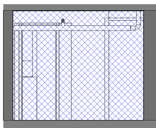
B0017 - Demolition Elevation C 1 : 50
