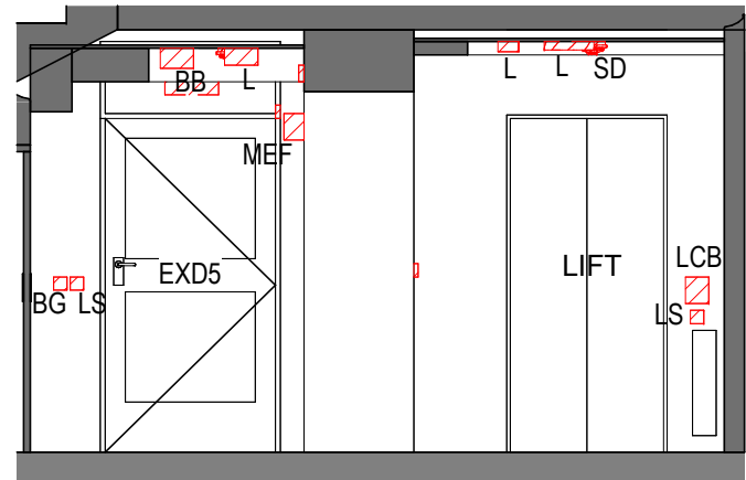
B0012 - Demolition Elevation D 1 : 50
