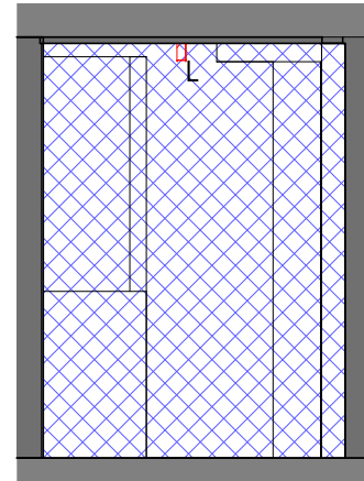
B0015 - Demolition Elevation C 1 : 50
