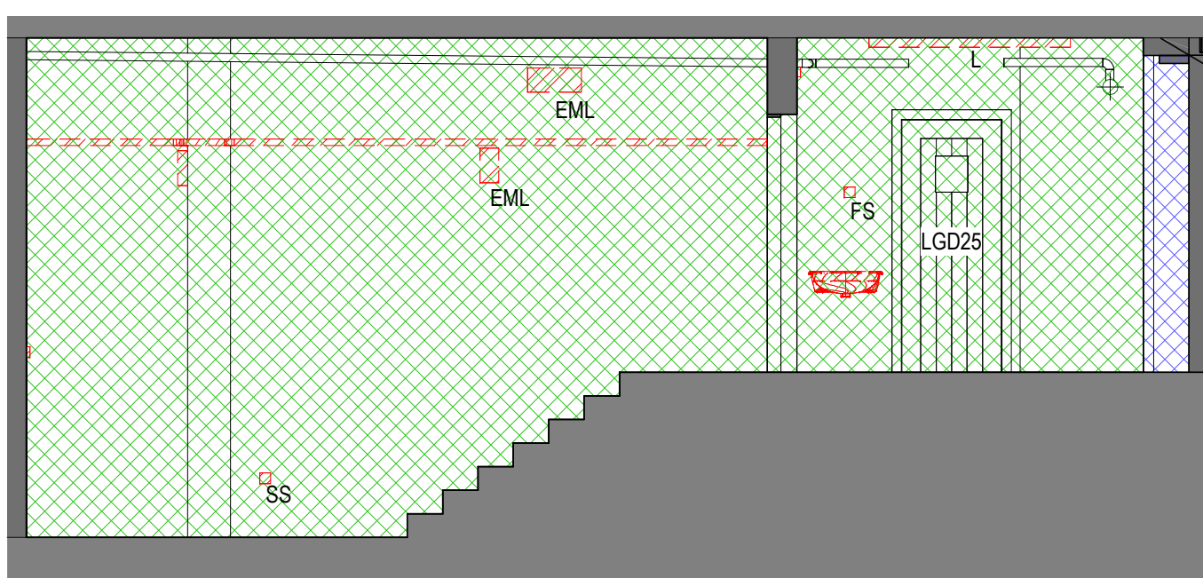
B0017 - Demolition Elevation B 1 : 50
