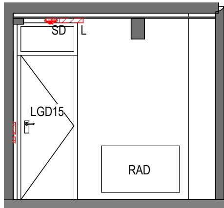
B0012 - Demolition Elevation A 1 : 50
