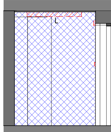
B0015 - Demolition Elevation D 1 : 50
