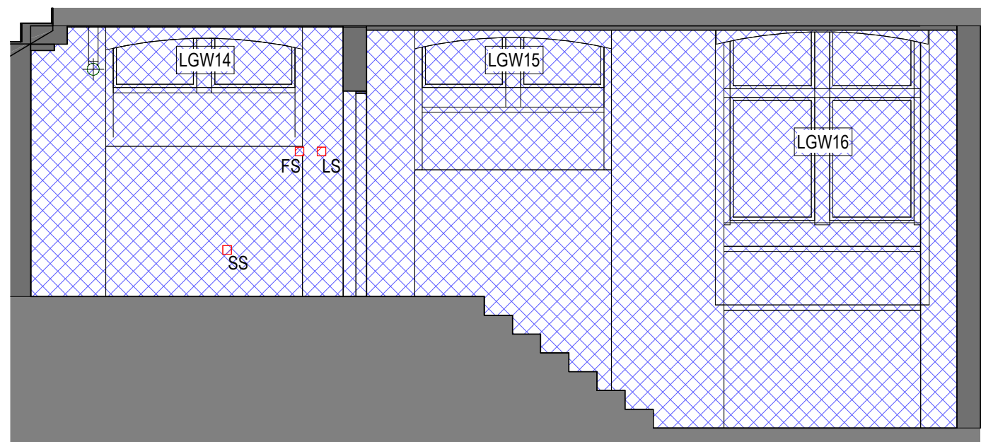
B0017 - Demolition Elevation D 1 : 50
