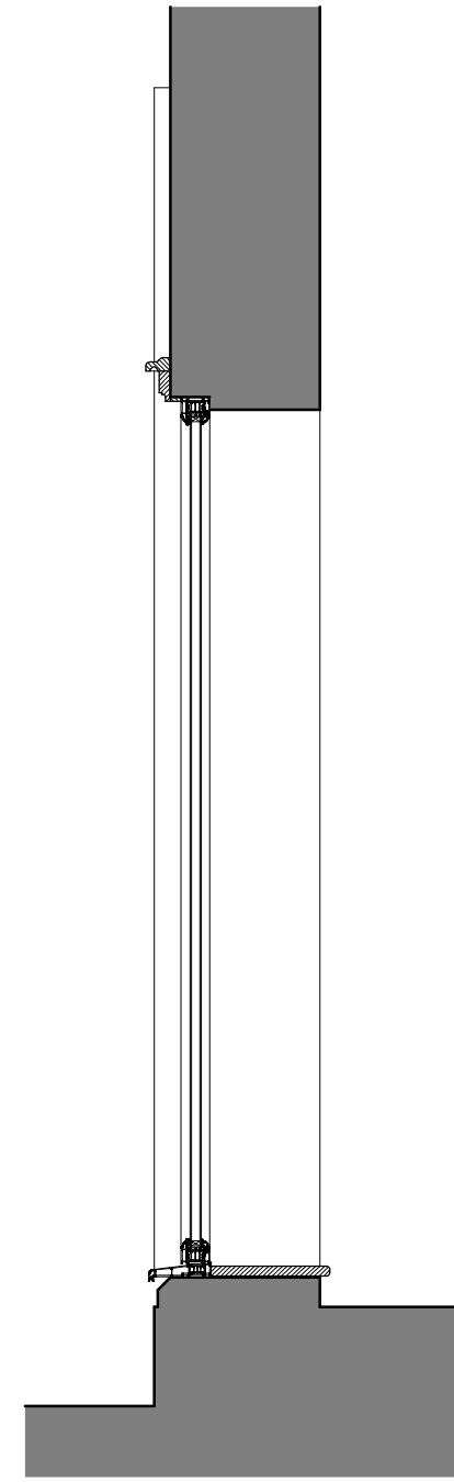
Cross Section (Left + Right Pane) SCALE 1:20
