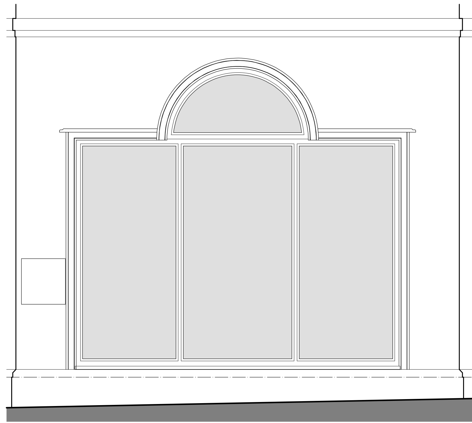
Roadside Elevation SCALE 1:20
