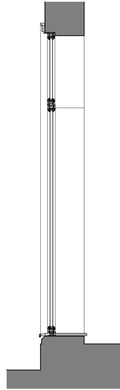
Cross Section (Centre Pane) SCALE 1:20
