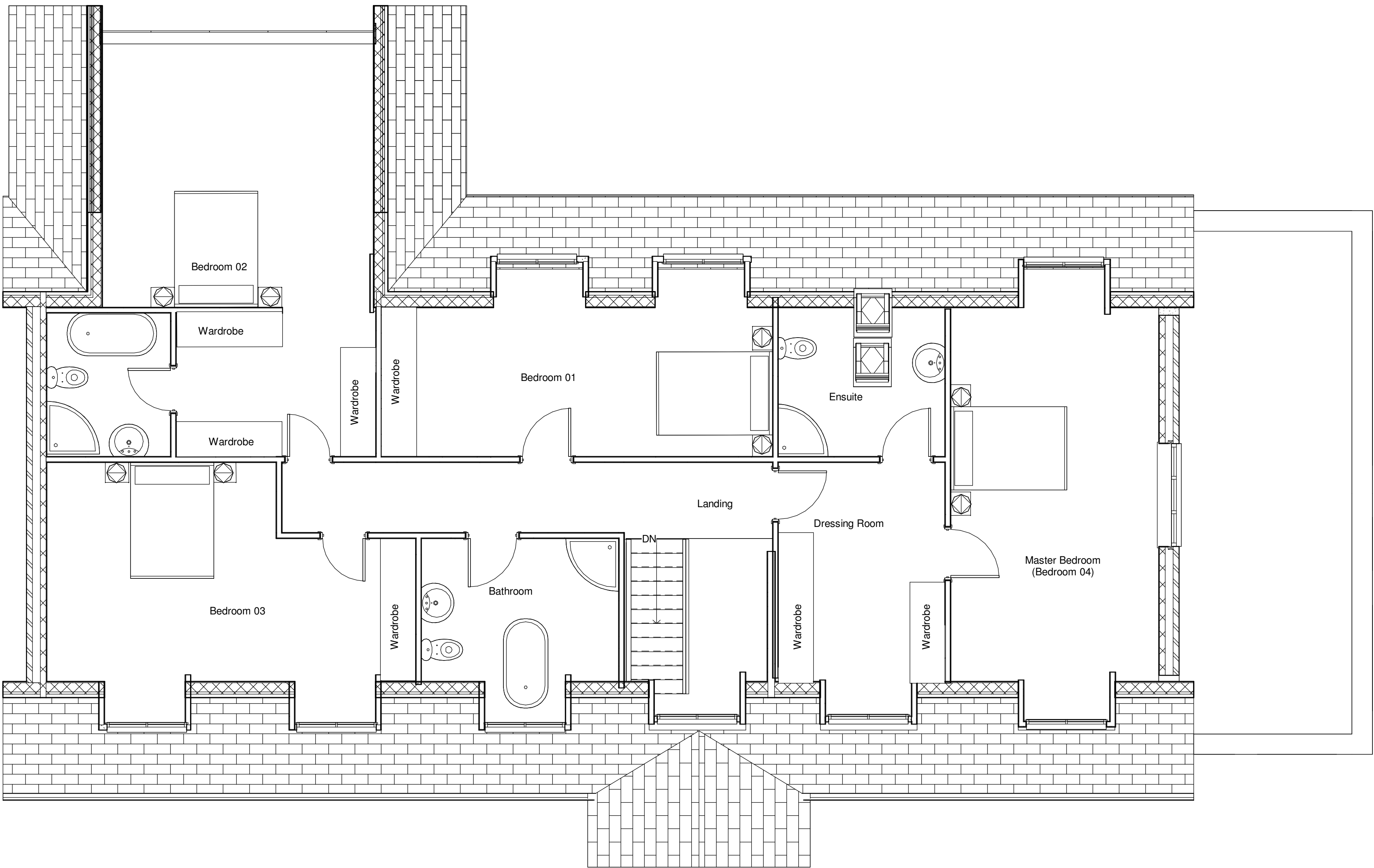
Proposed FF Plan 1 : 50
