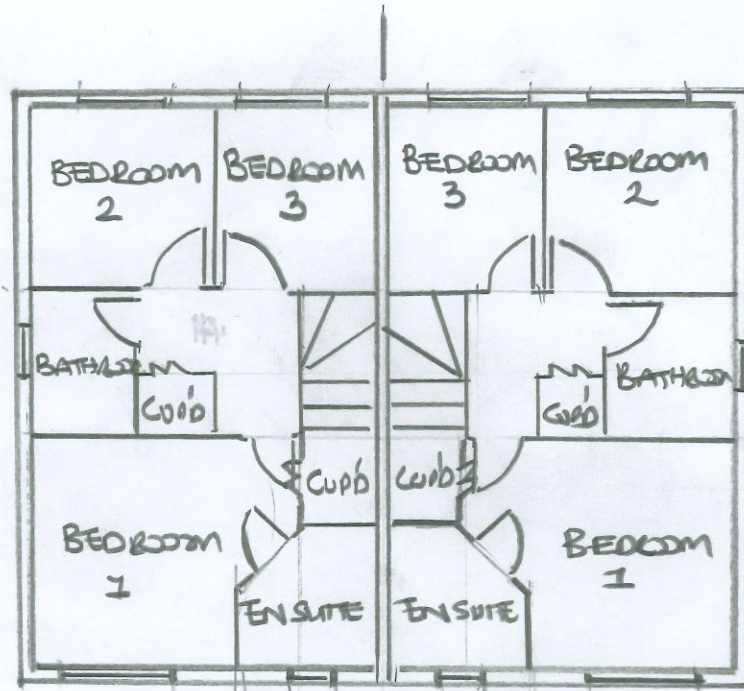
FIRST FLOOR LAYOUT.
