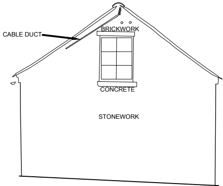
ELEVATION 2 OUTBUILDING 04
