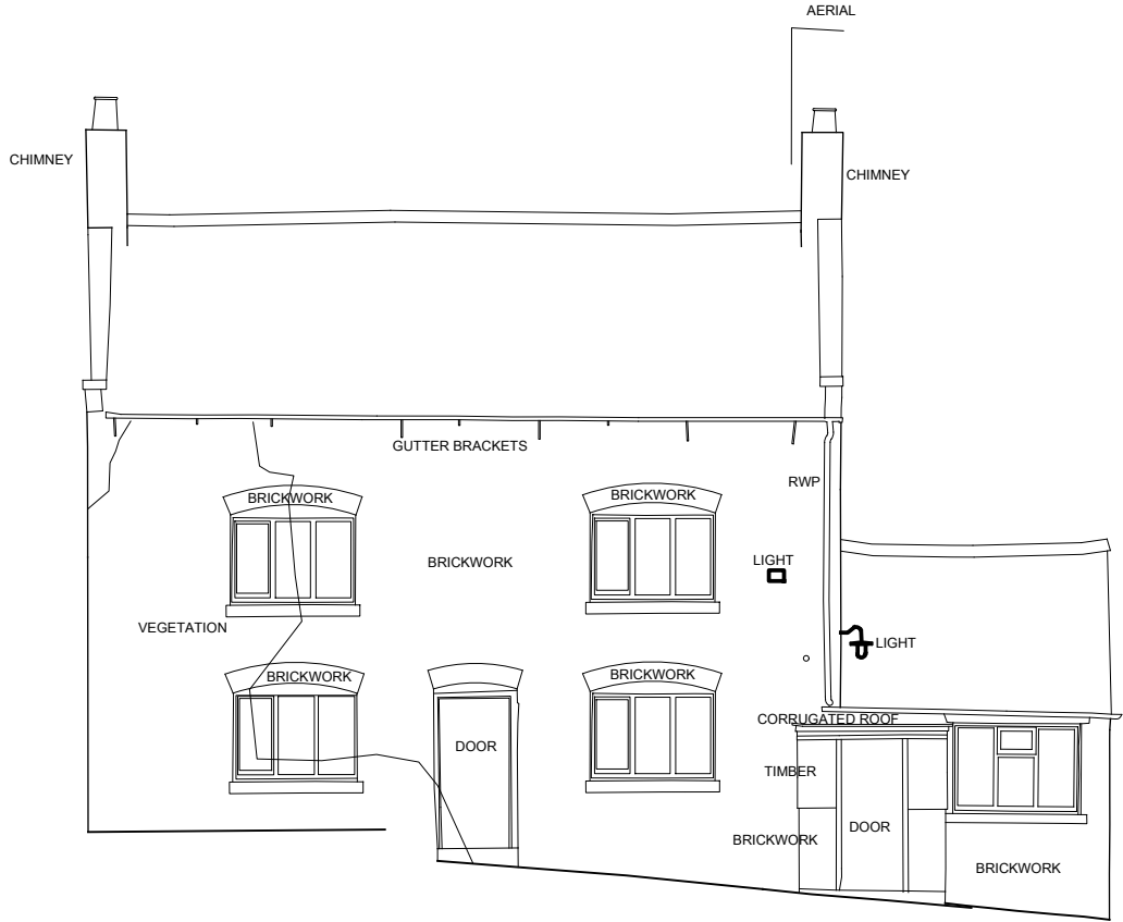
ELEVATION 1 FARMHOUSE
