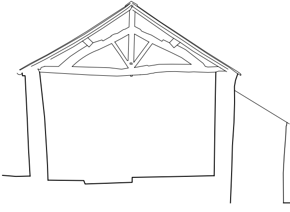
SECTION E-E OUTBUILDING 04
