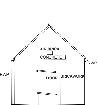
ELEVATION 1 OUTBUILDING 03
