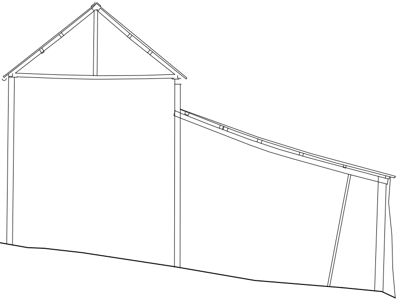
SECTION F-F OUTBUILDING 05
