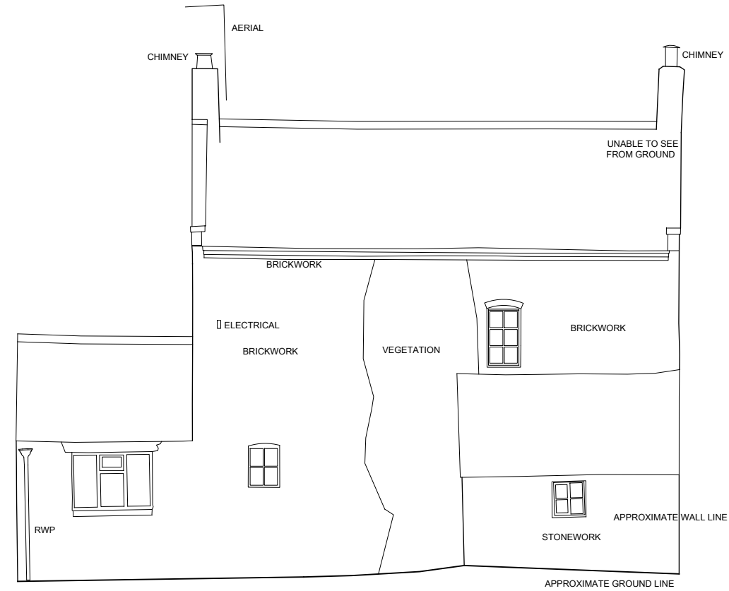
ELEVATION 3 FARMHOUSE
