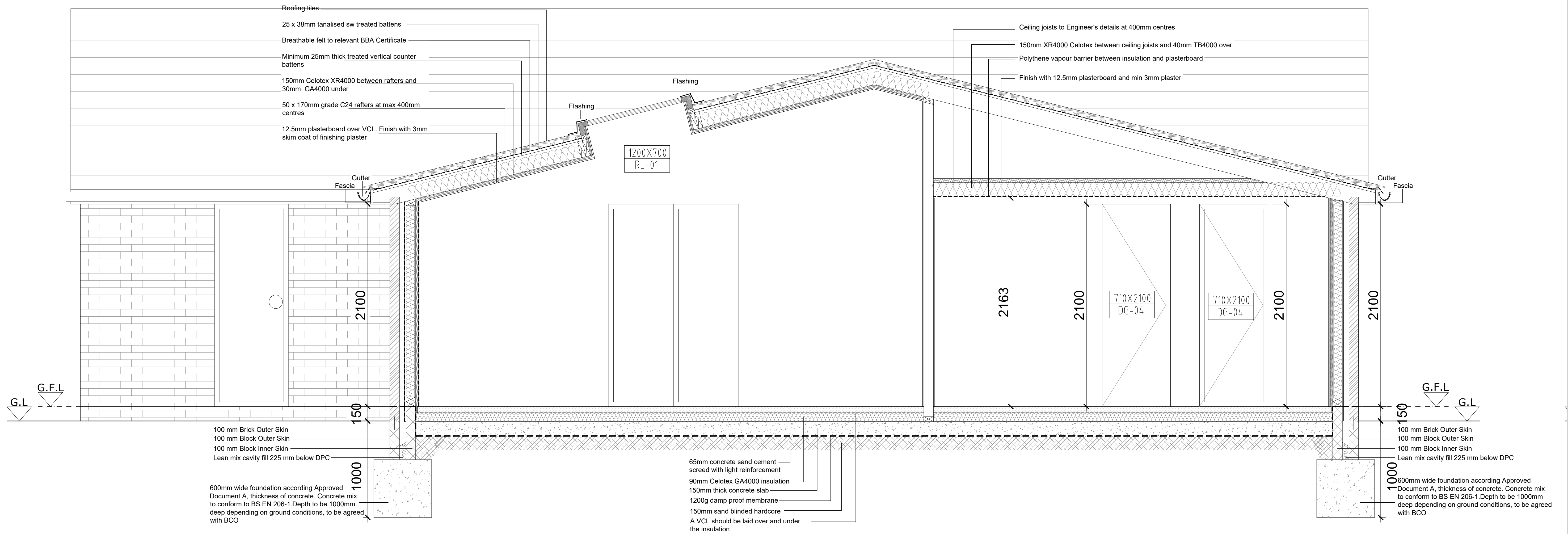
SECTION AA (SCALE 1:20)
