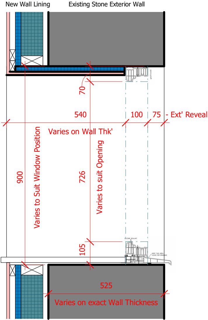
Window - Vertical Section 1 : 10
