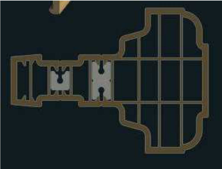
Central Mullion Profile
