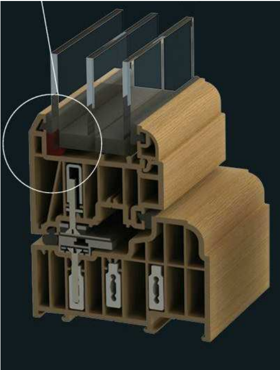
Flush Casement - Frame Profile
