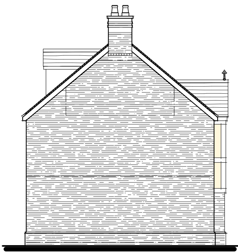
South Elevation
