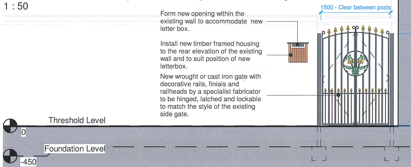
Rear Elevation of Proposed Wrought / Cast iron gate 1 : 50
