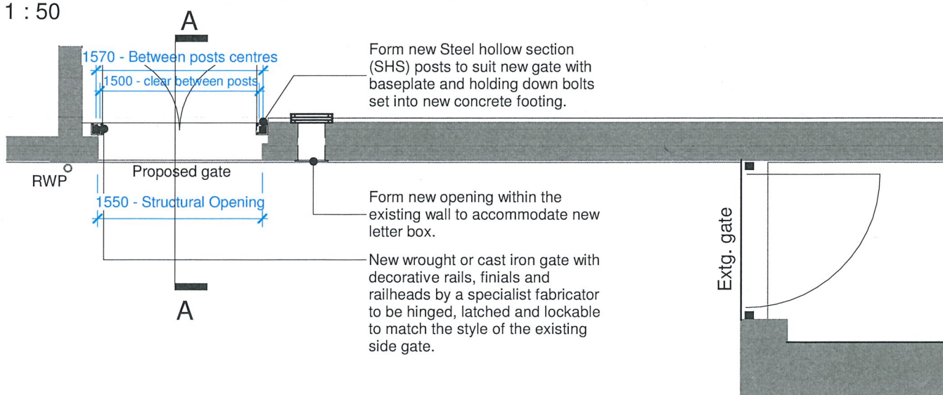
Plan as Proposed 1 : 50
