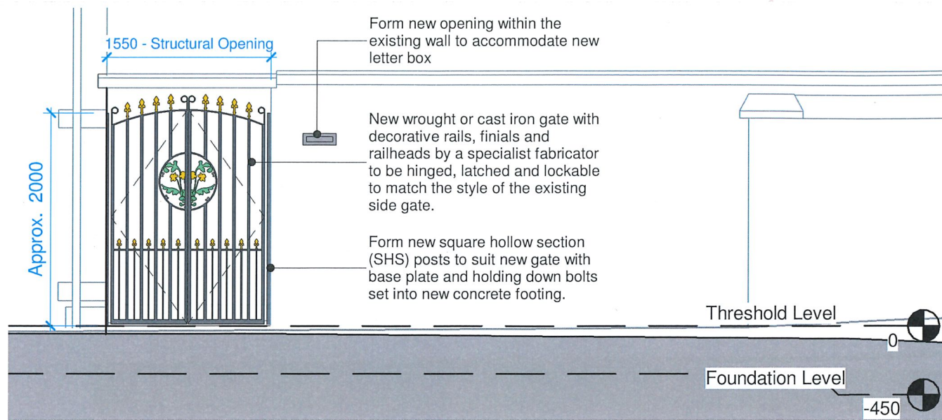
Front Elevation of Proposed Wrought / Cast iron gate 1 : 50
