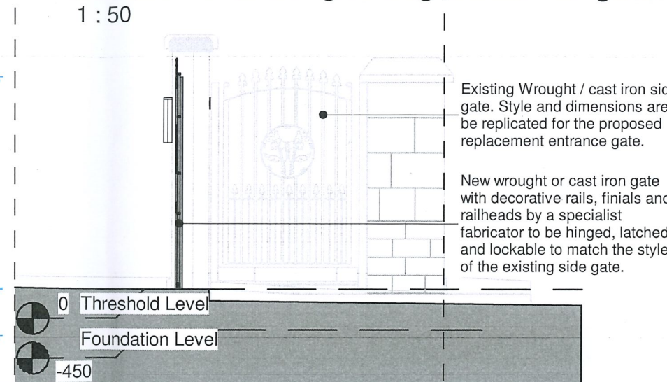
Section A through Proposed gate 1 : 50
