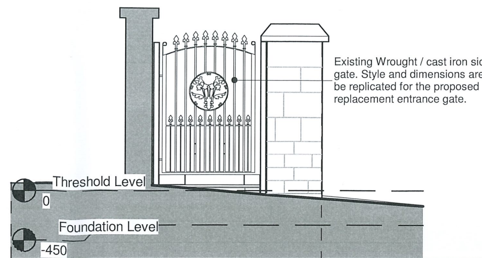
Elevation of Existing Wrought/Cast iron gate 1 : 50
