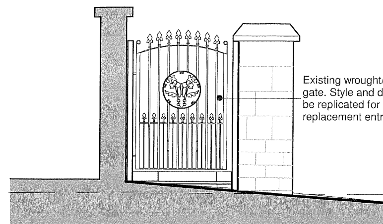
Elevation of Existing Wrought/Cast iron gate 1 : 50
