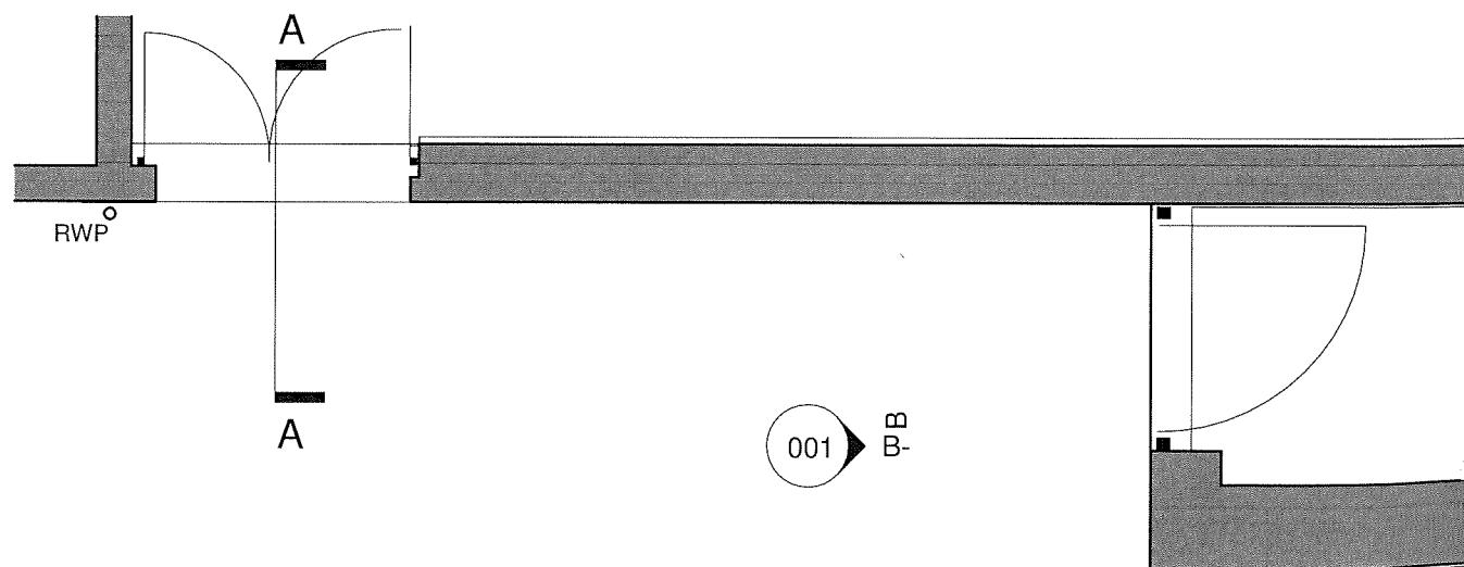
Plan as Existing 1 : 50
