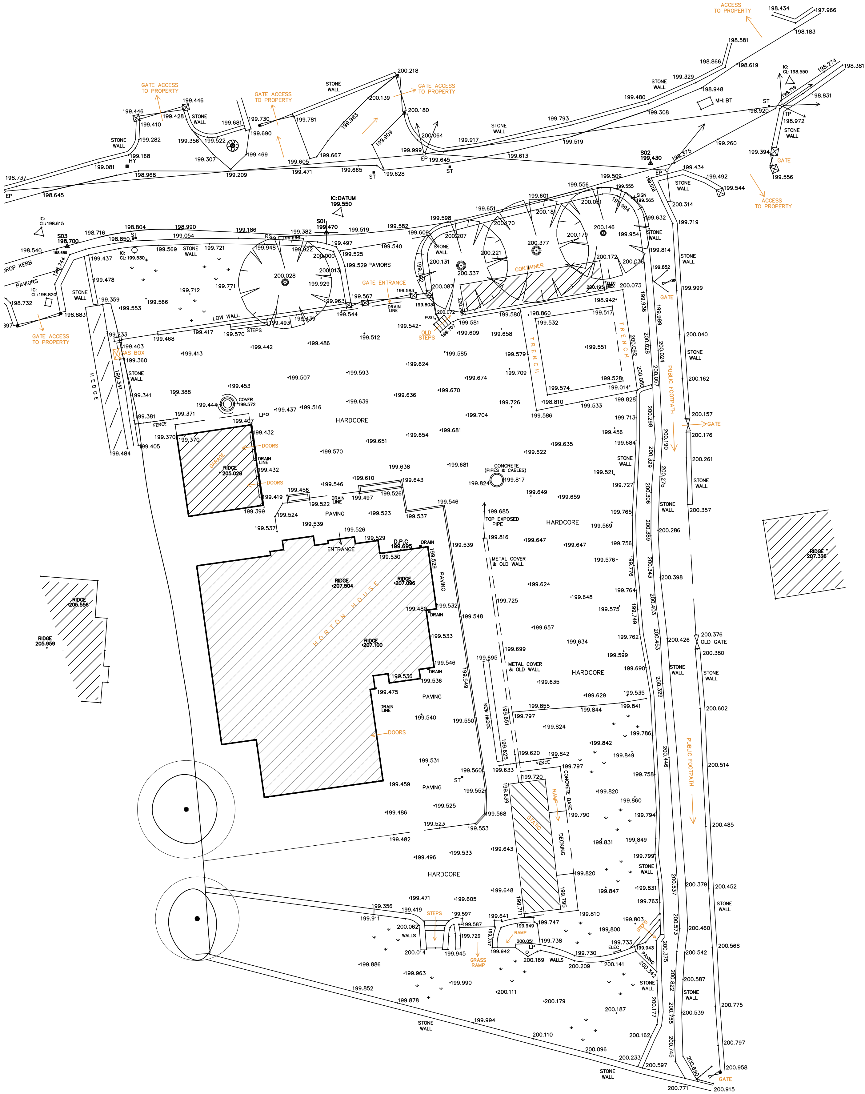
Existing Site Layout Plan 1:200
