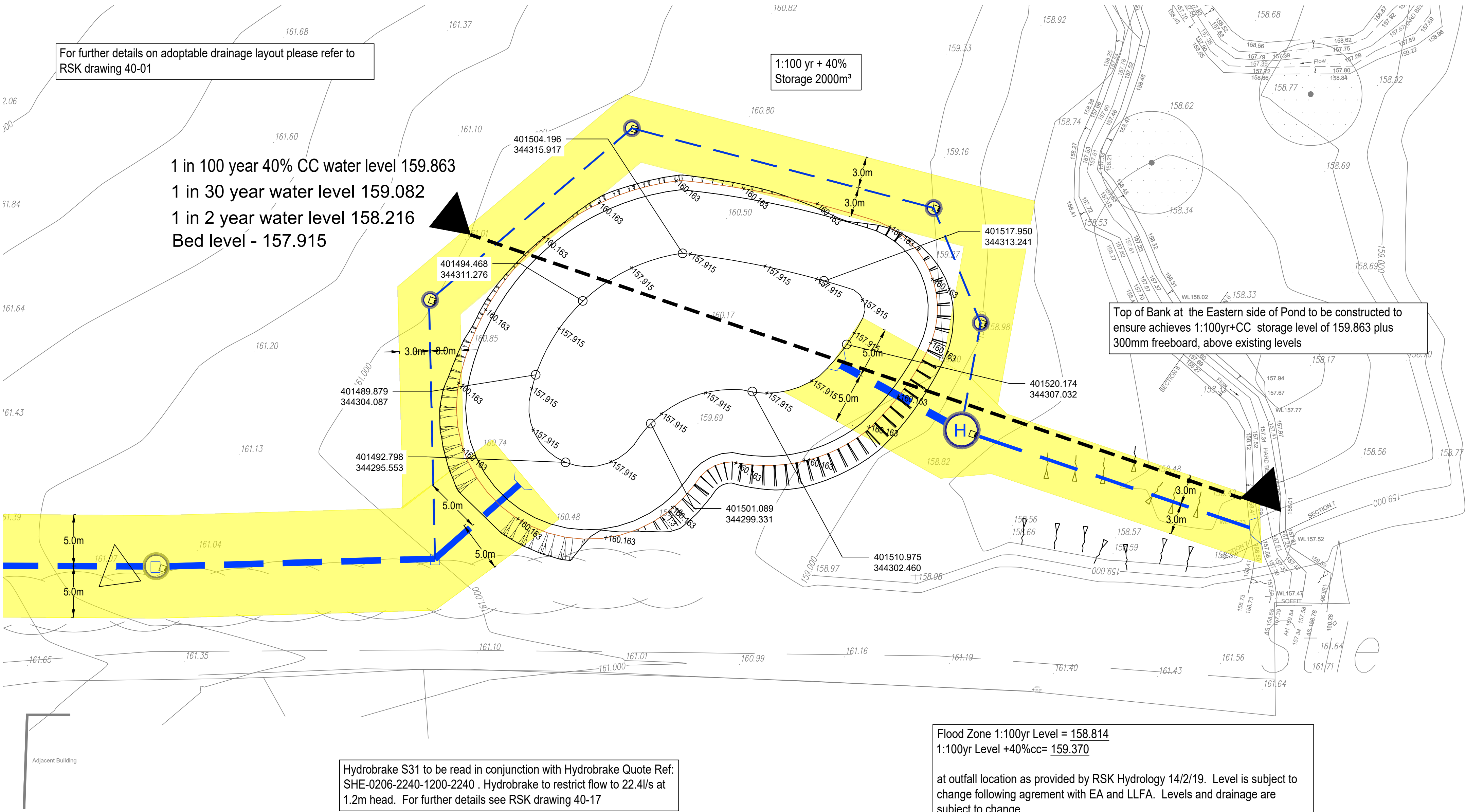
Basin Plan Scale 1:250
