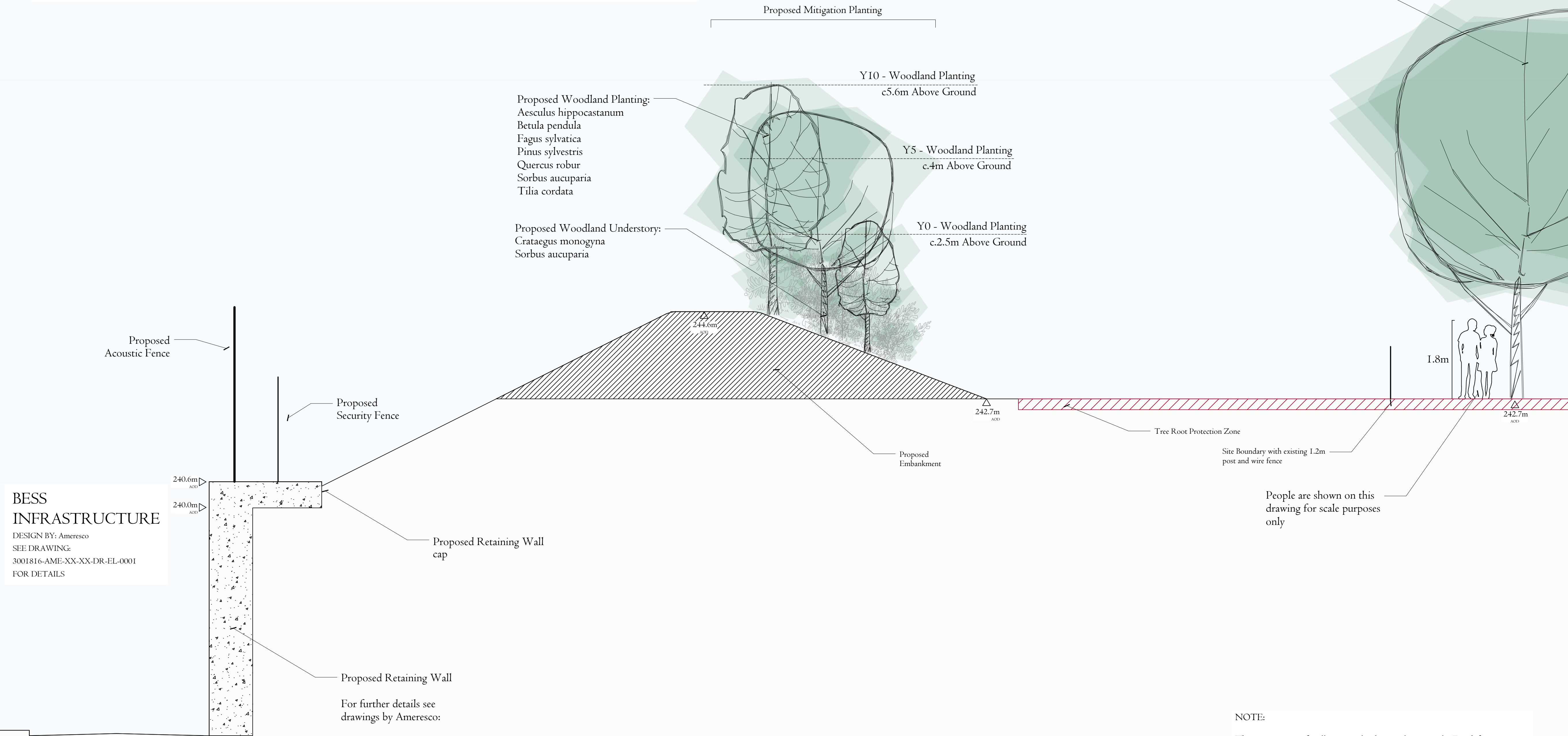
Section A-A North
