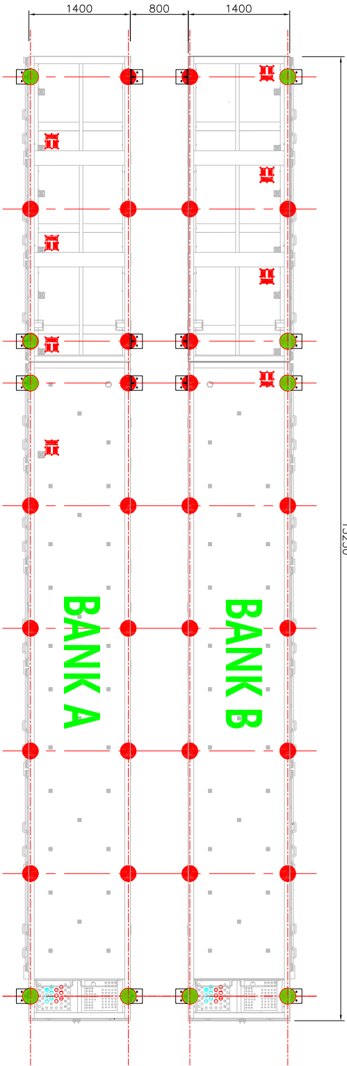
Installation diagram on the TOP VIEW of BankA&B
