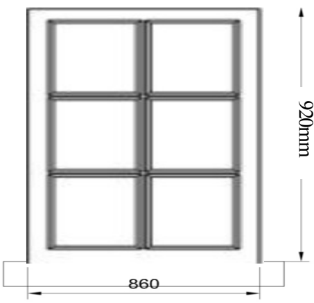
EXTERNAL ELEVATION
