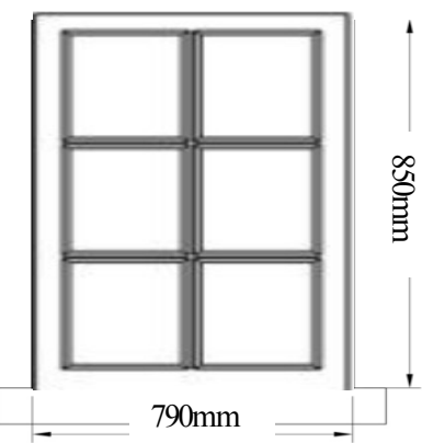
EXTERNAL ELEVATION
