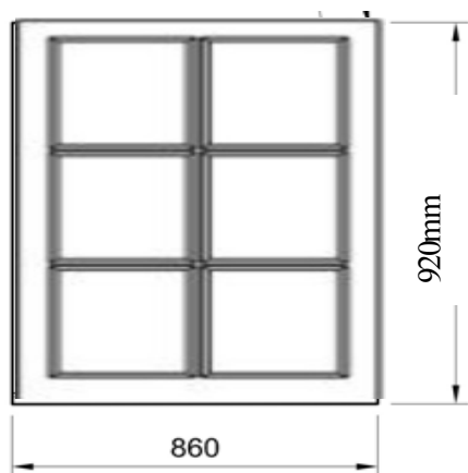
EXTERNAL ELEVATION
