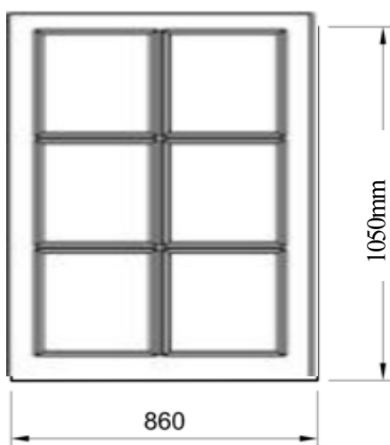
EXTERNAL ELEVATION
