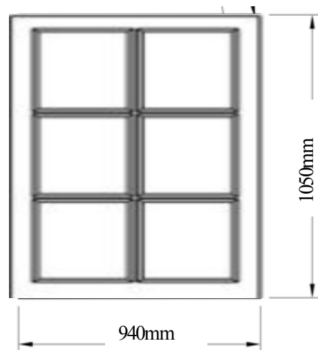
EXTERNAL ELEVATION
