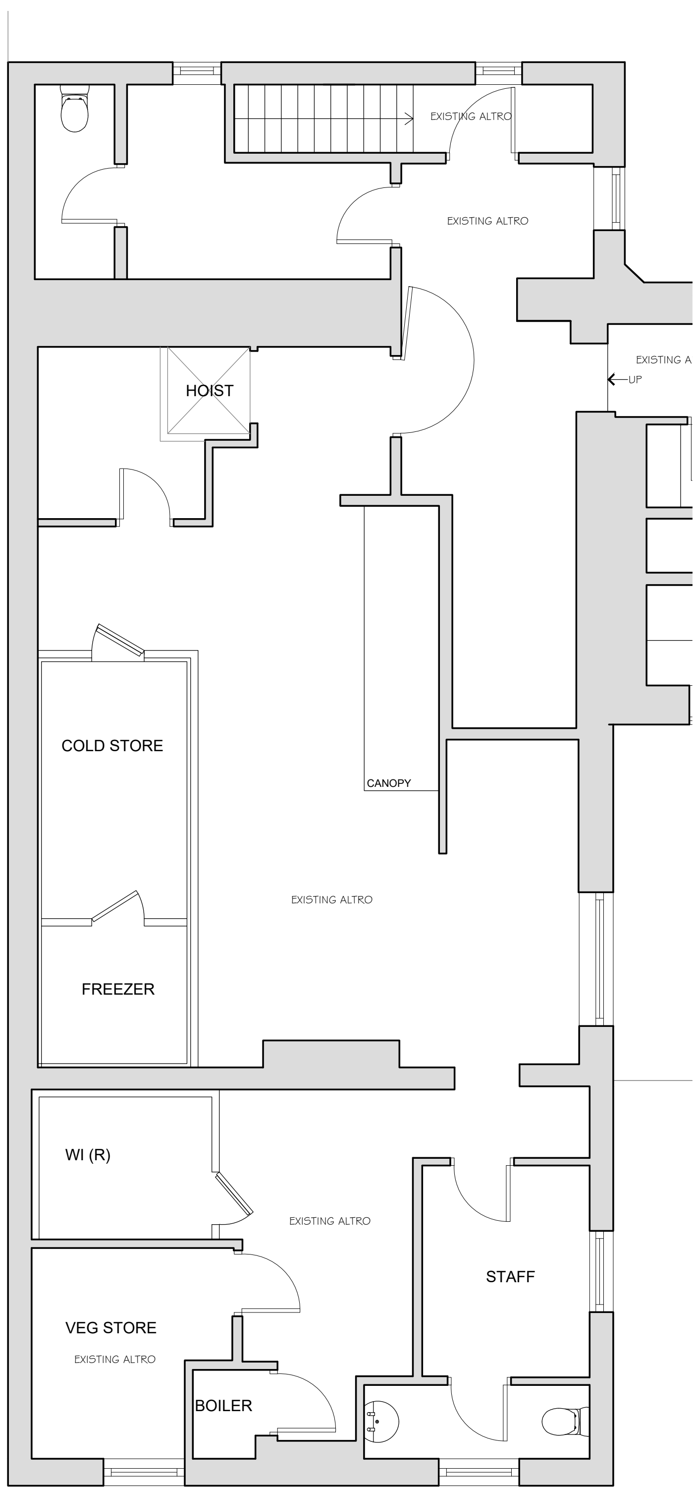
FIRST FLOOR KITCHEN
