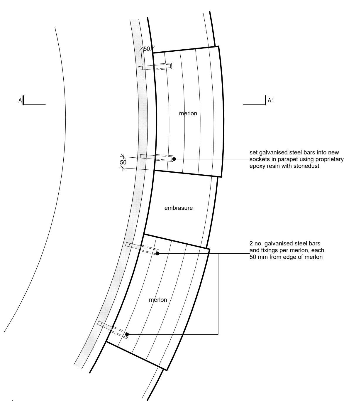
detail A new handrail to roof terrace
