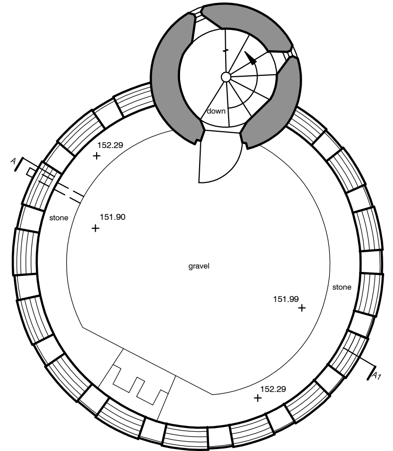
Roof Plan
