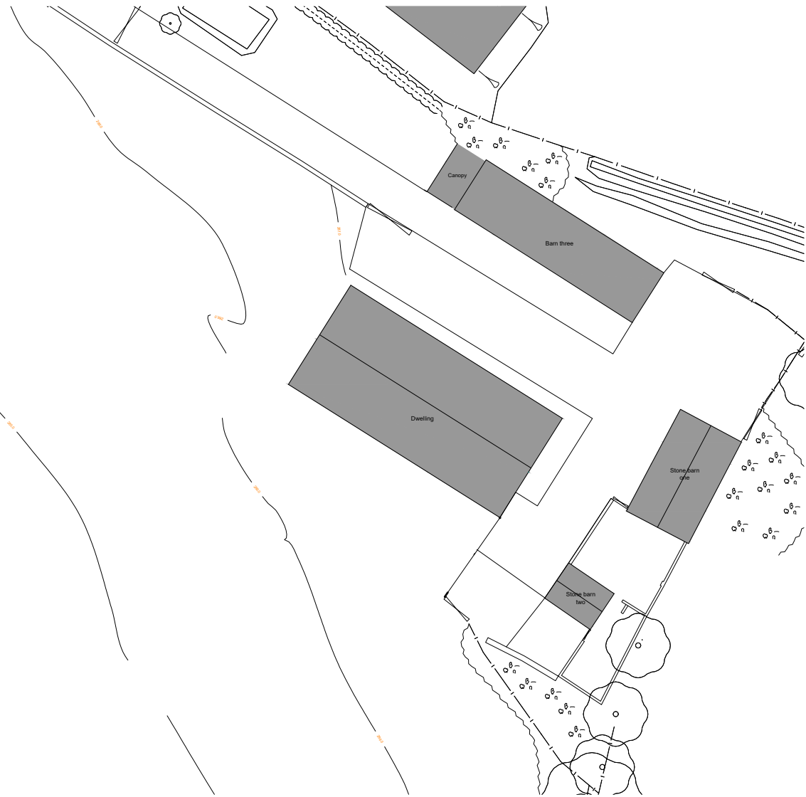
Context plan 1:500
