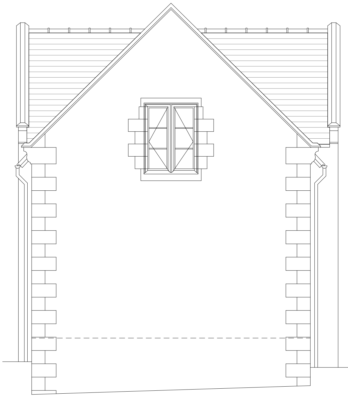
SOUTH-WEST ELEVATION
