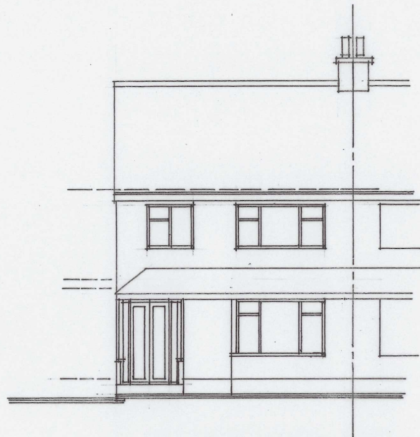
EXISTING FRONT ELEVATION ( WEST )
