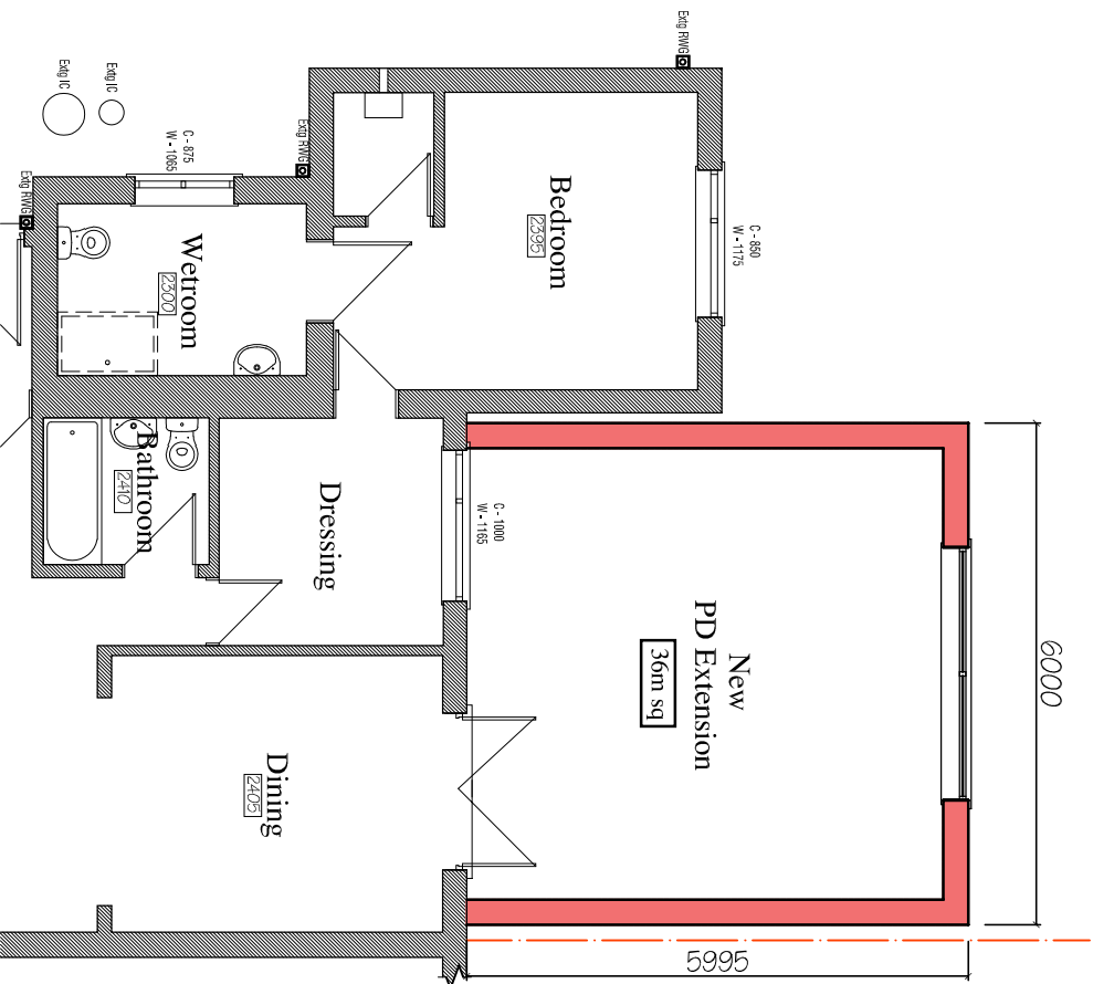
Proposed Plan
