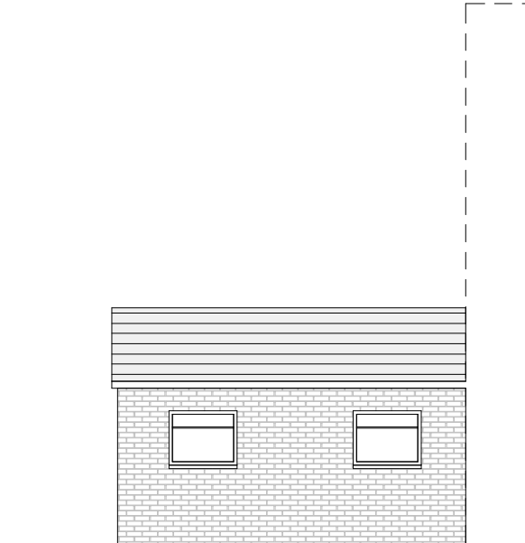
6 West Elevation 1 : 100
