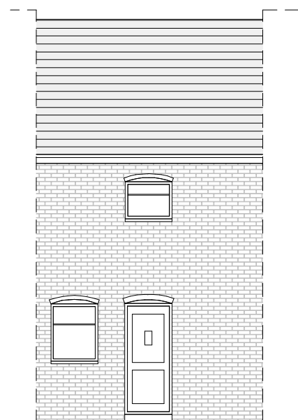
3 South Elevation 1 : 100
