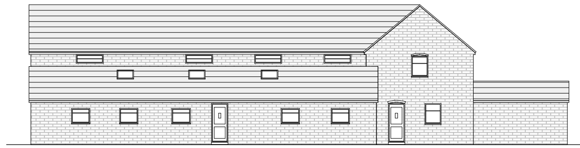
4 East Elevation 1 : 200
