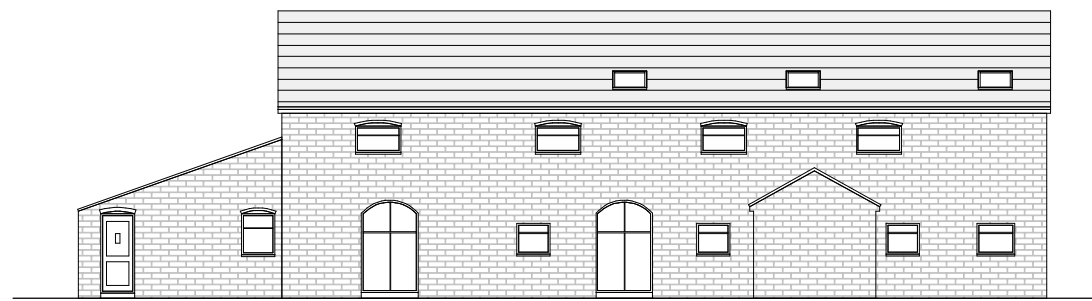
5 North Elevation 1 : 200
