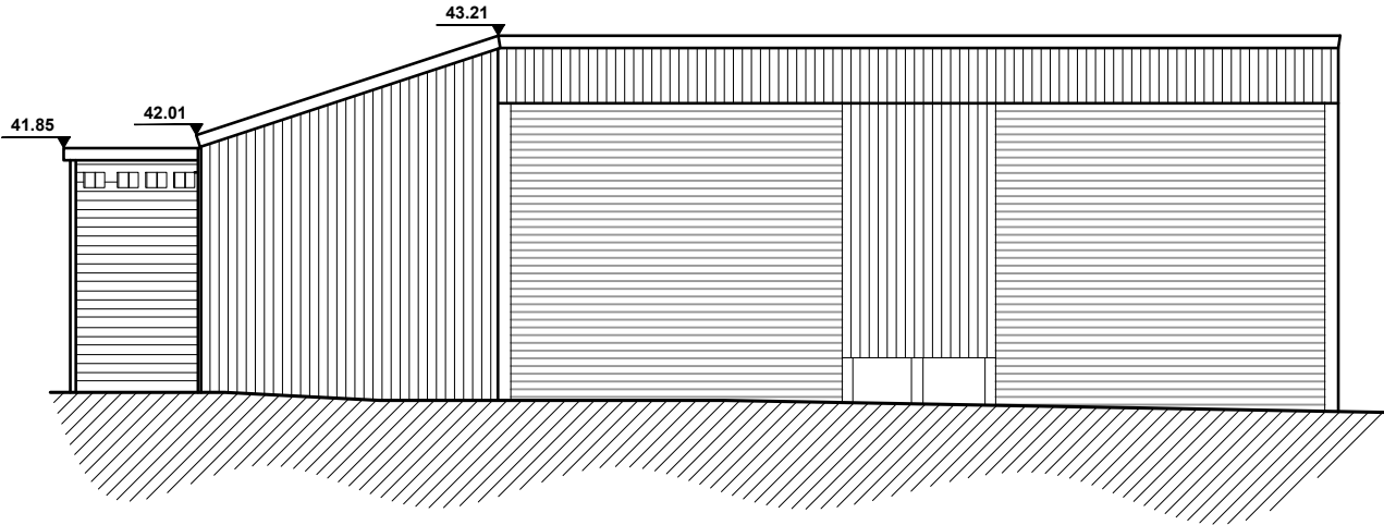
3. Rear Elevation (North)
