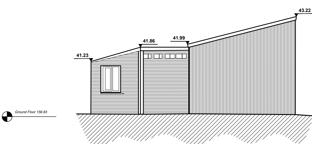
4. Side Elevation (West)
