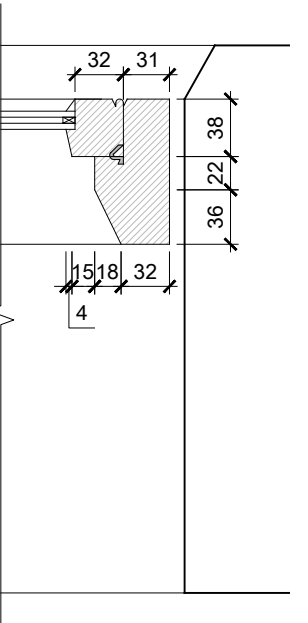
CASEMENT WINDOW - JAMB DETAIL: 1:5 SECTION F-F
