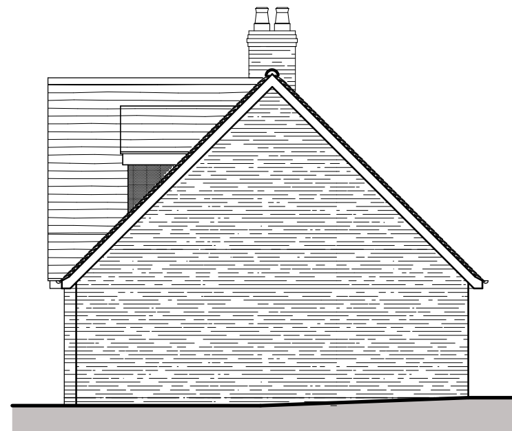
South Elevation
