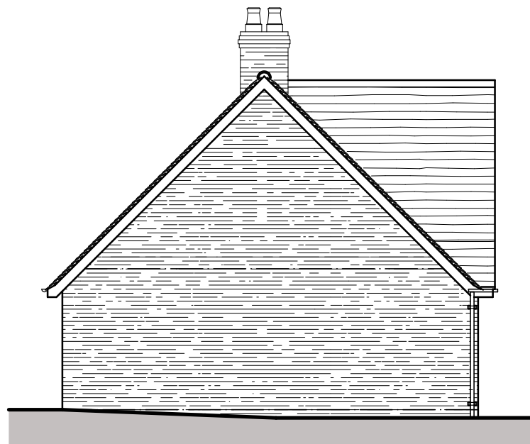
North Elevation
