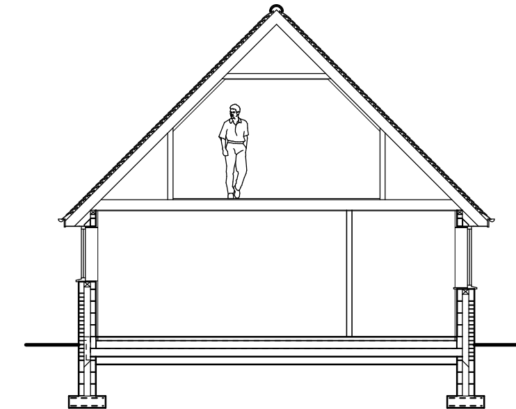
Section
