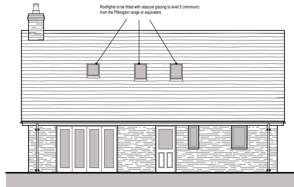
North Elevation
