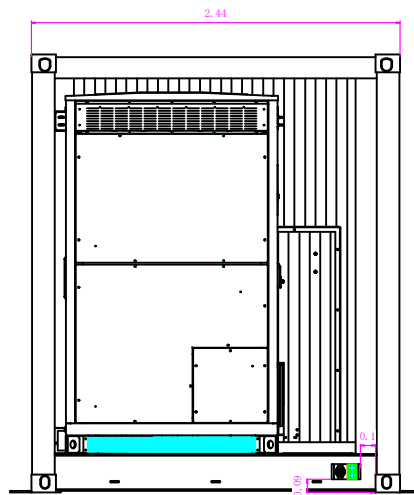
Left View
