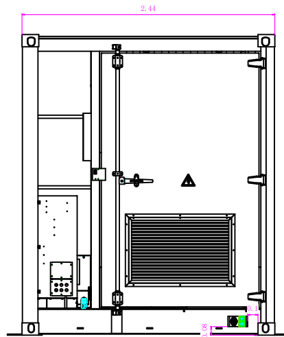
Right View
