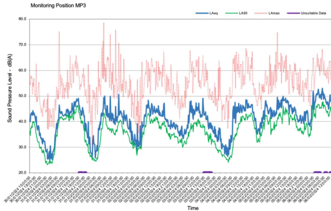
Figure 7-8 Measured Time History – MP3 – Statistical Analysis - Day
