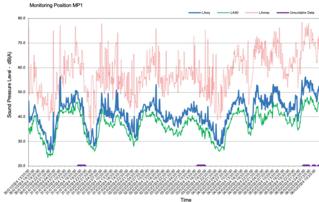
Figure 7-1 Measured Time History – MP1 – Whole Period
