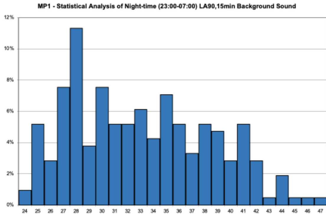
Figure 7-3 Measured Time History – MP1 – Statistical Analysis - Night
