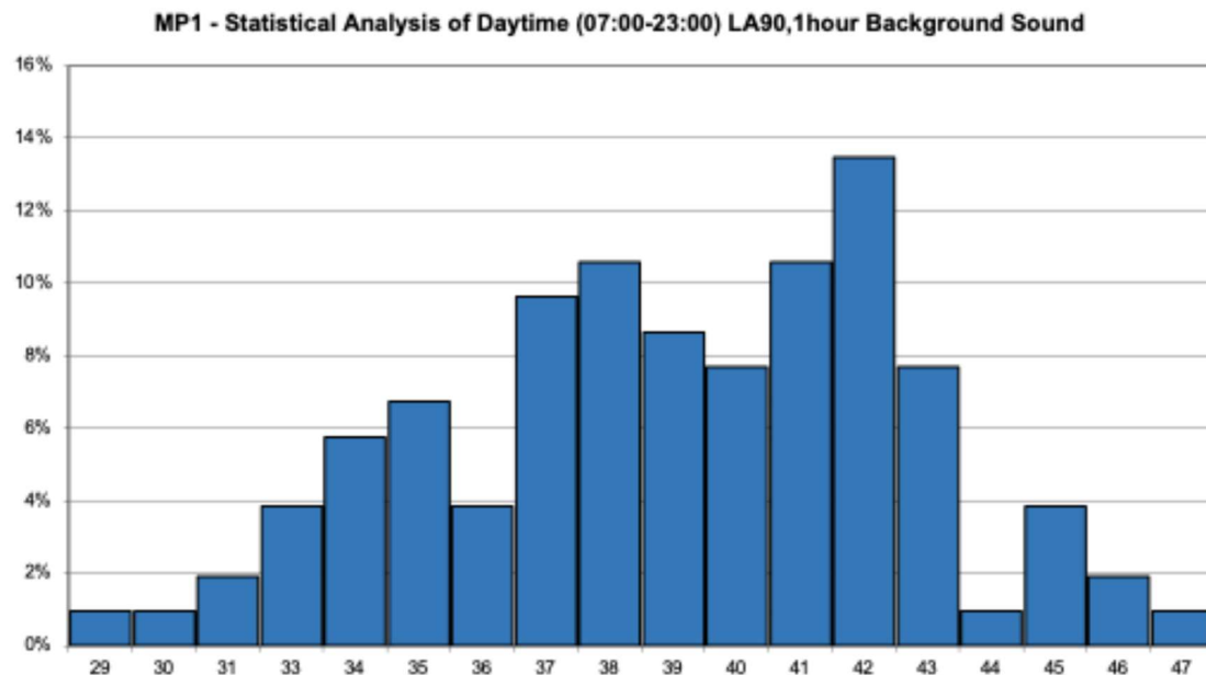
Figure 7-2 Measured Time History – MP1 – Statistical Analysis - Day
