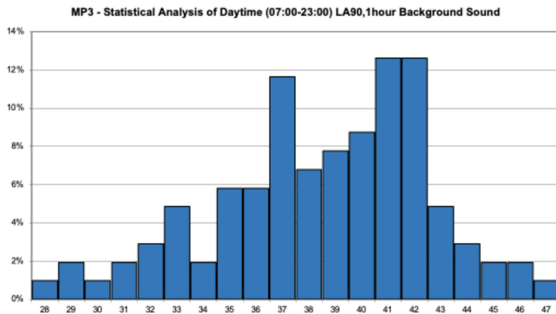
Figure 7-8 Measured Time History – MP3 – Statistical Analysis - Day
