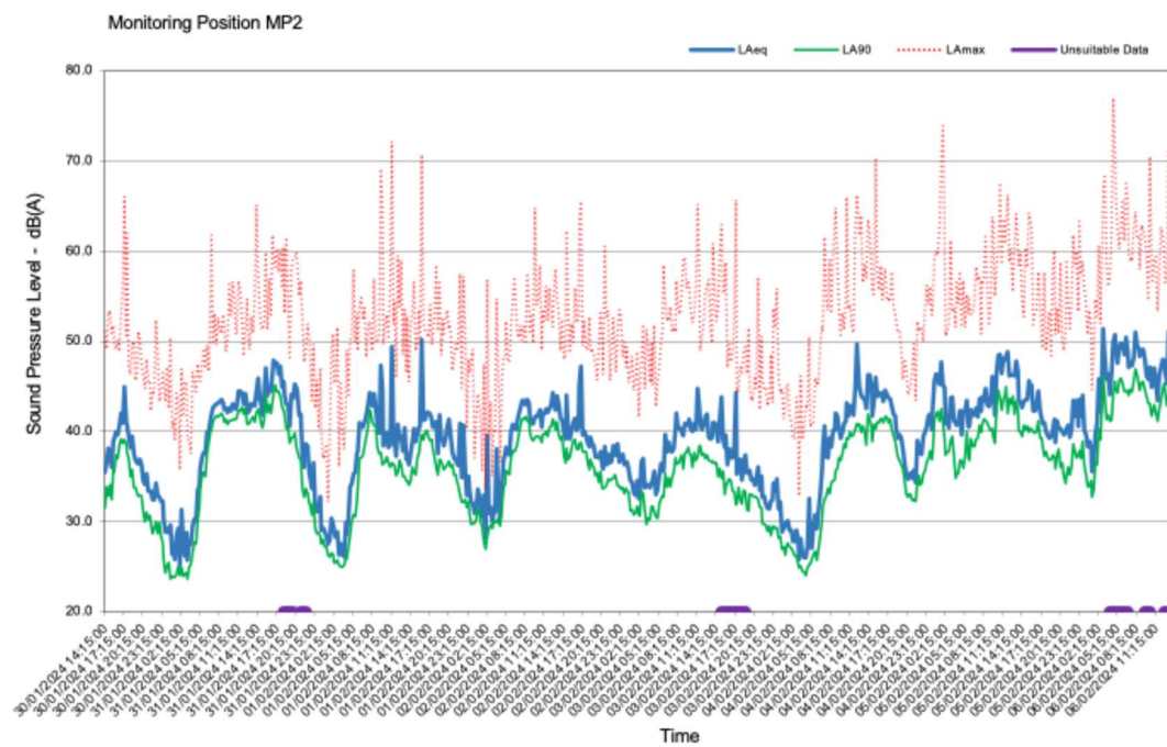
Figure 7-4 Measured Time History – MP2 – Whole Period
