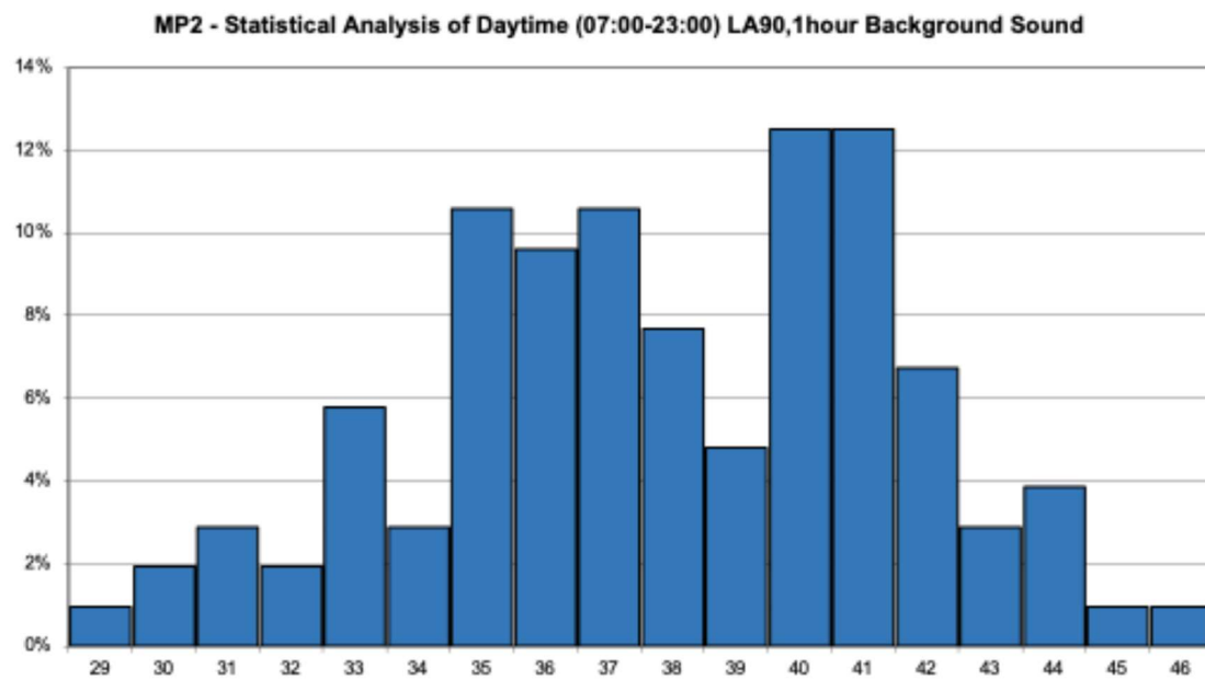
Figure 7-5 Measured Time History – MP2 – Statistical Analysis - Day
