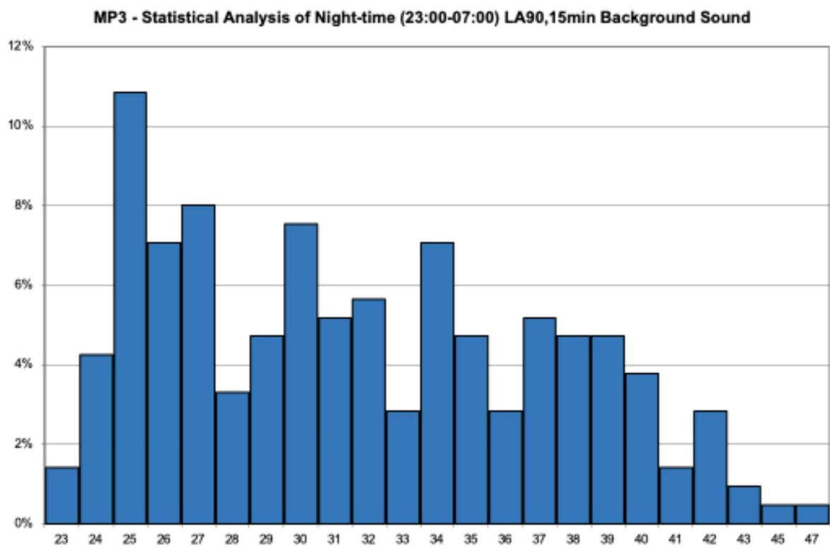
Figure 7-9 Measured Time History – MP3 – Statistical Analysis - Night
