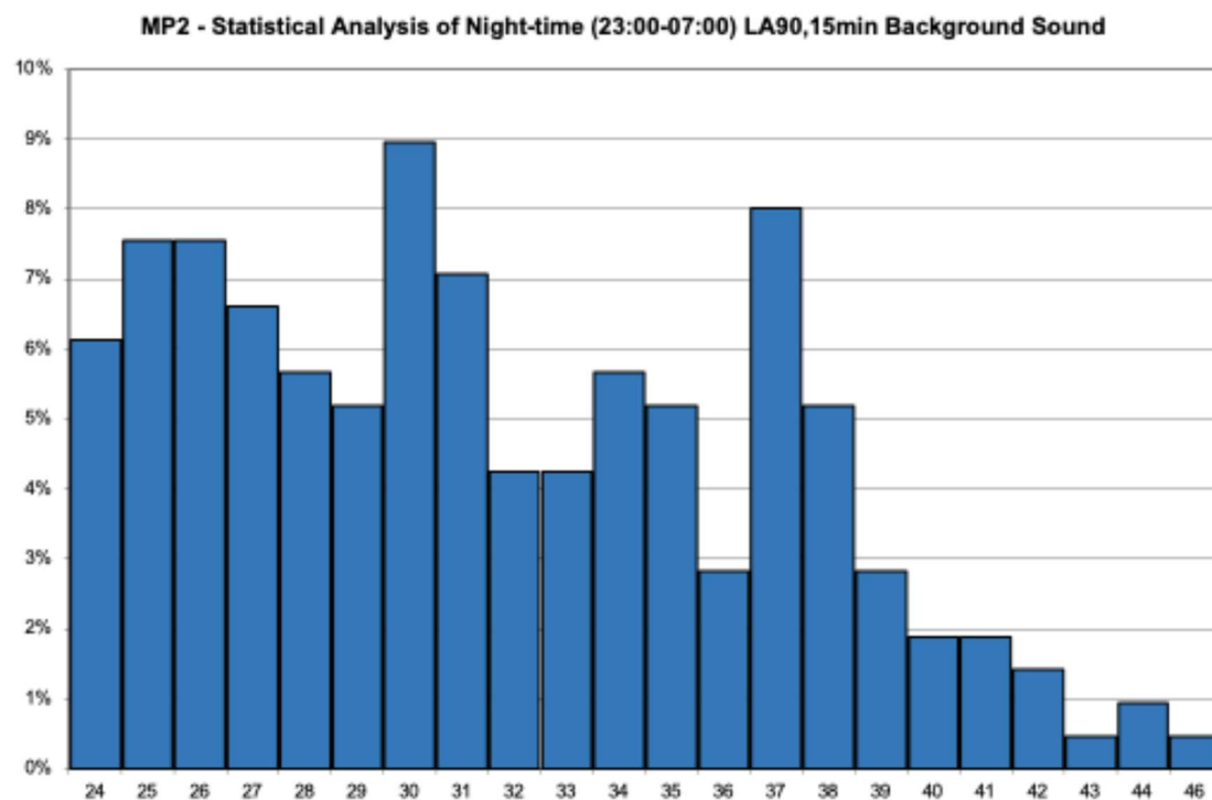
Figure 7-6 Measured Time History – MP2 – Statistical Analysis - Night
