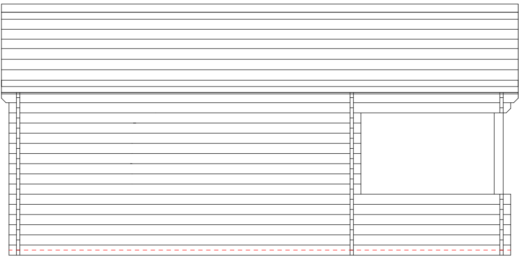
Side Elevation 1
