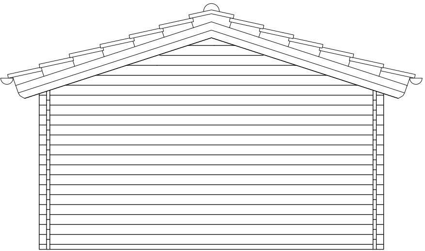
Back Elevation
