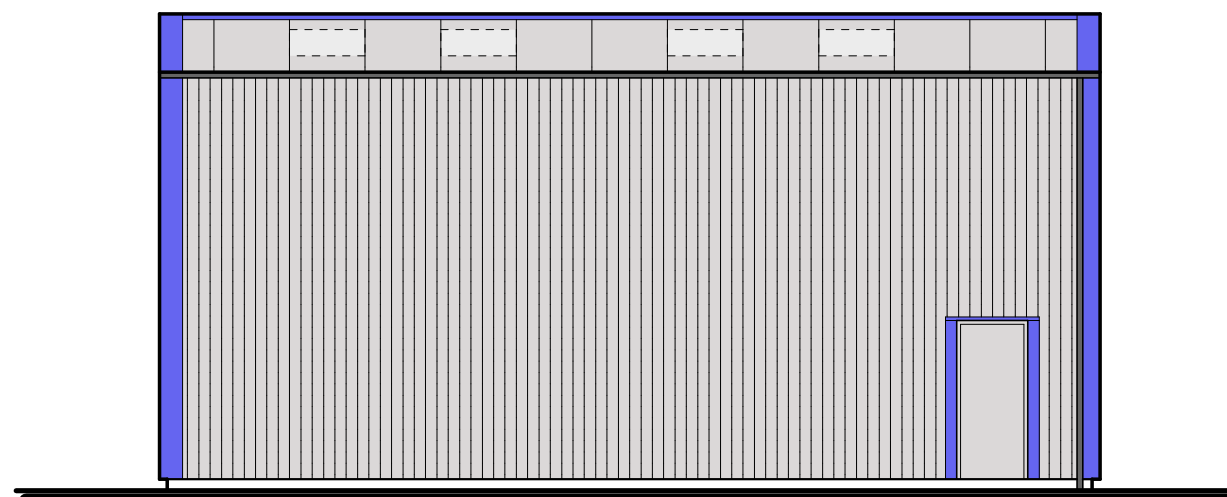
East Elevation
