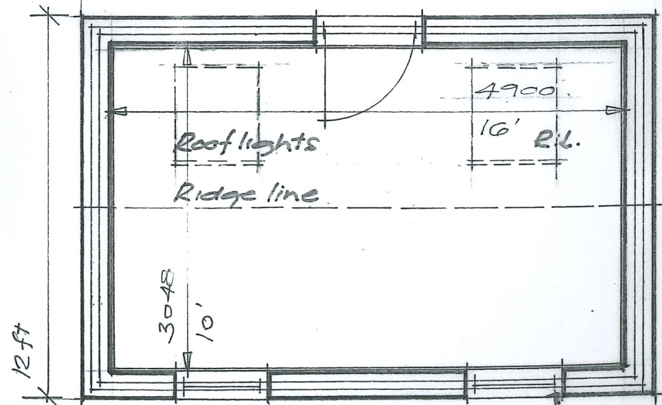
Floor Plan 1:50 0 1 2 3 4 5m.
