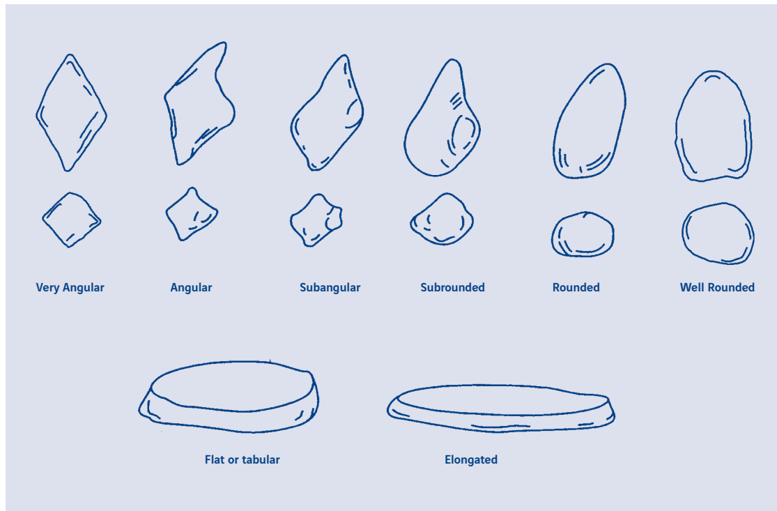
FIGURE 1: PARTICLE ANGULARITY AND FORM TERMS (from BS 5930: 2015 + A1 2020 and Soil Engineering)
