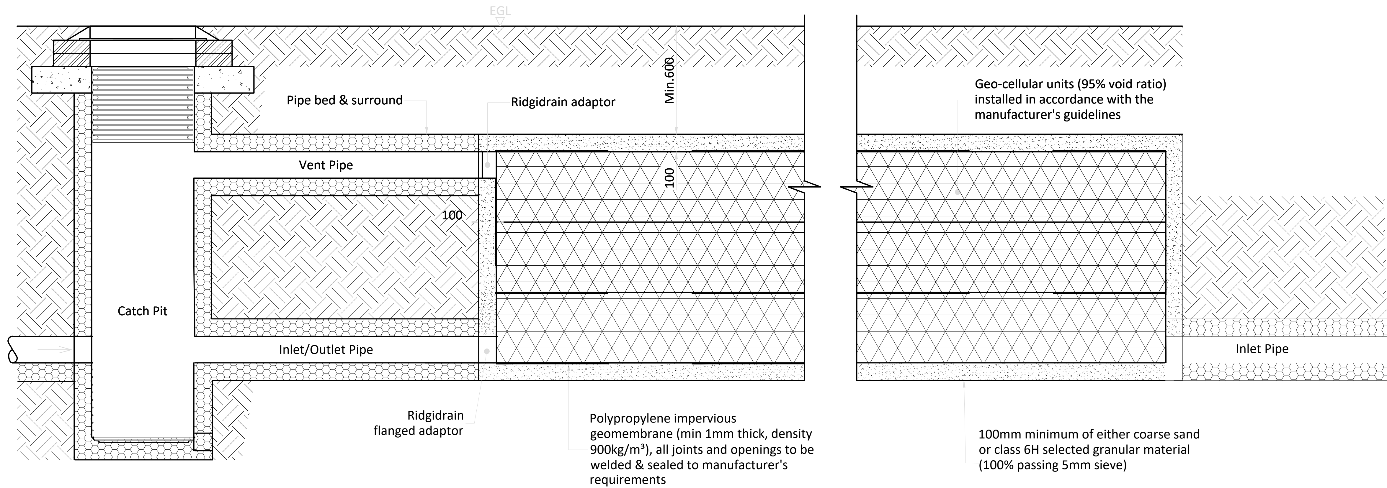
Section Through Storm Water Attenuation Crates
