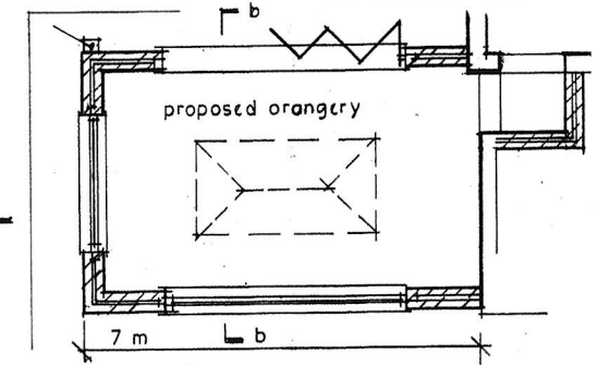
1:50 ORANGERY PLAN
