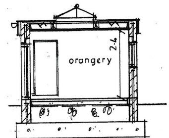
1:50 SECTION B-B
