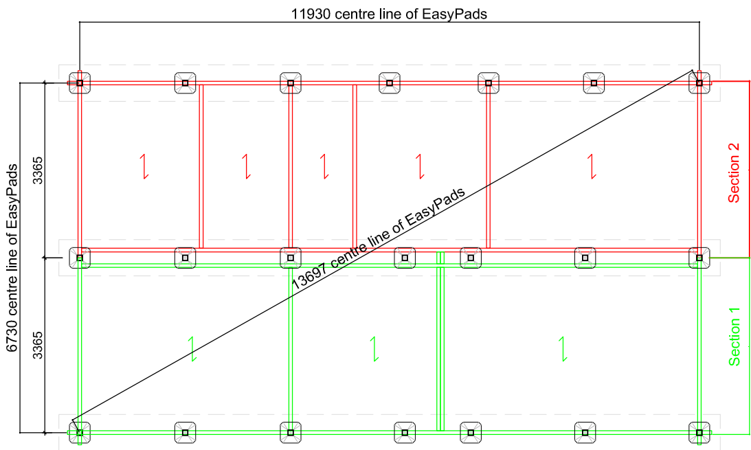
EasyPad Layout
