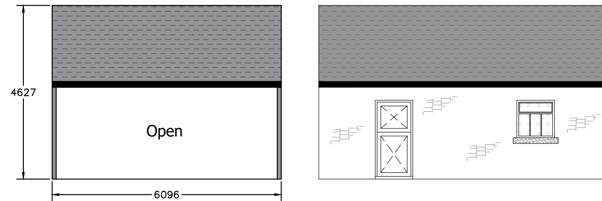
East Side Elevation
