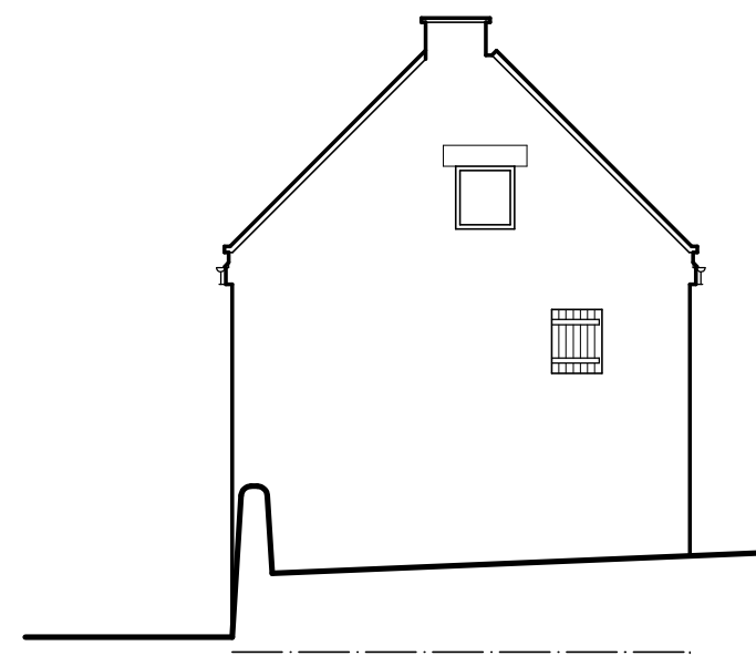
East Elevation
