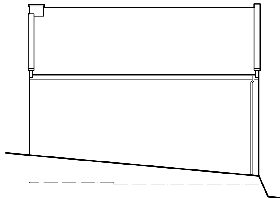
South Elevation
