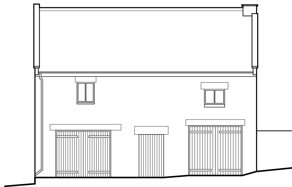
North Elevation
