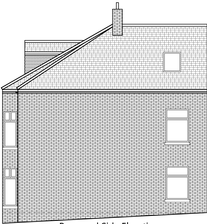
Proposed Side Elevation John Street
