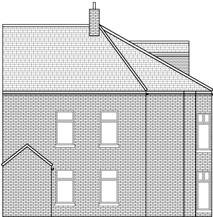
Existing Rear Elevation Garden
