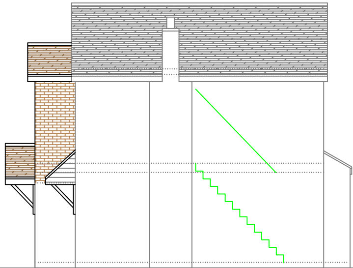
Side Elevation
