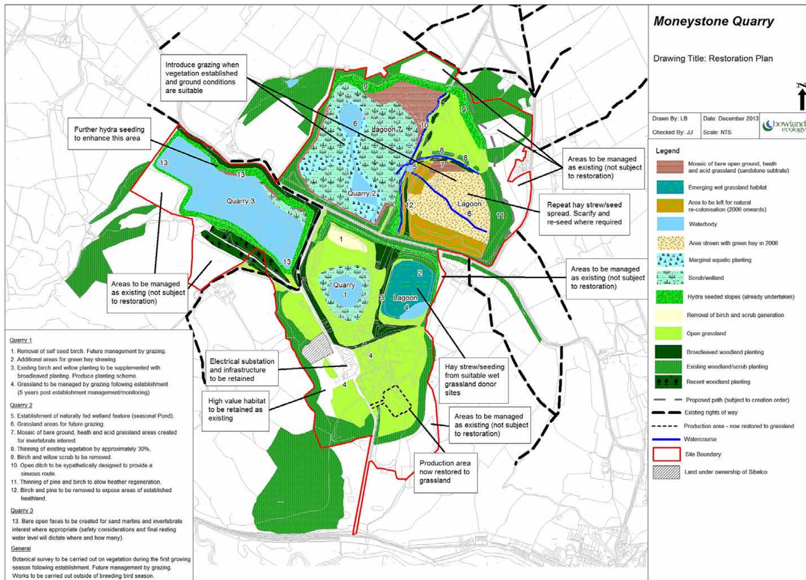
FIGURE 8.2: RESTORATION PLAN
