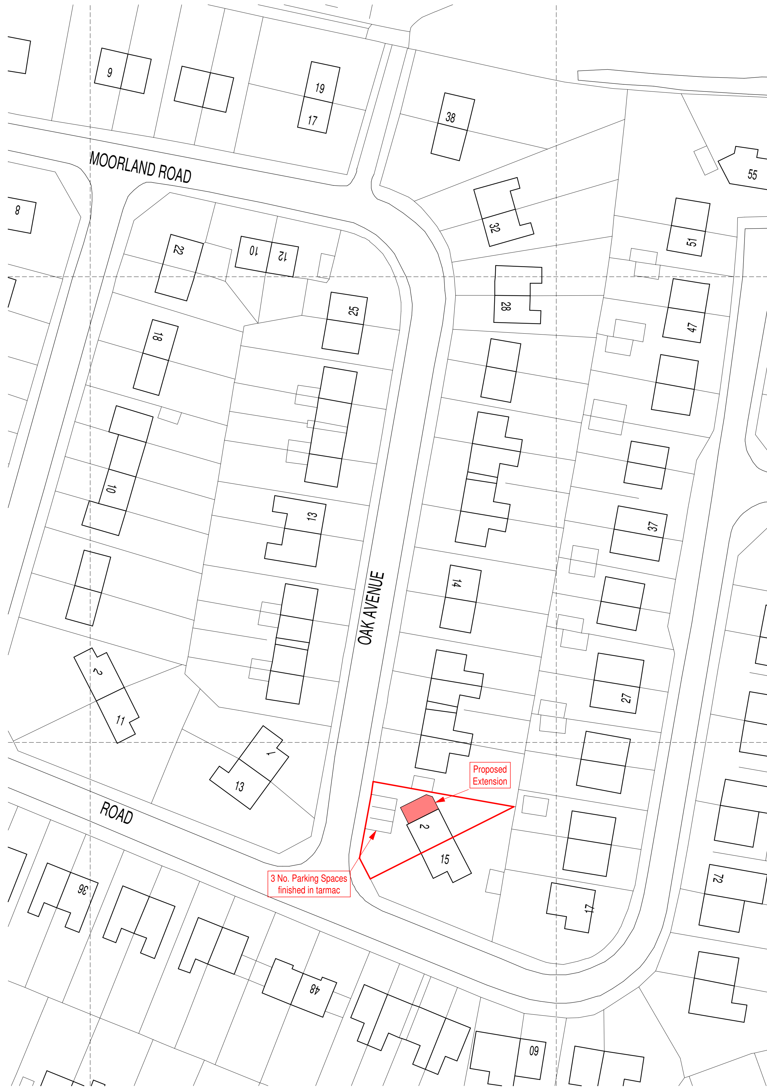
Block Plan
