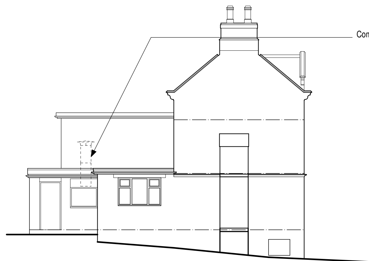
West Elevation
