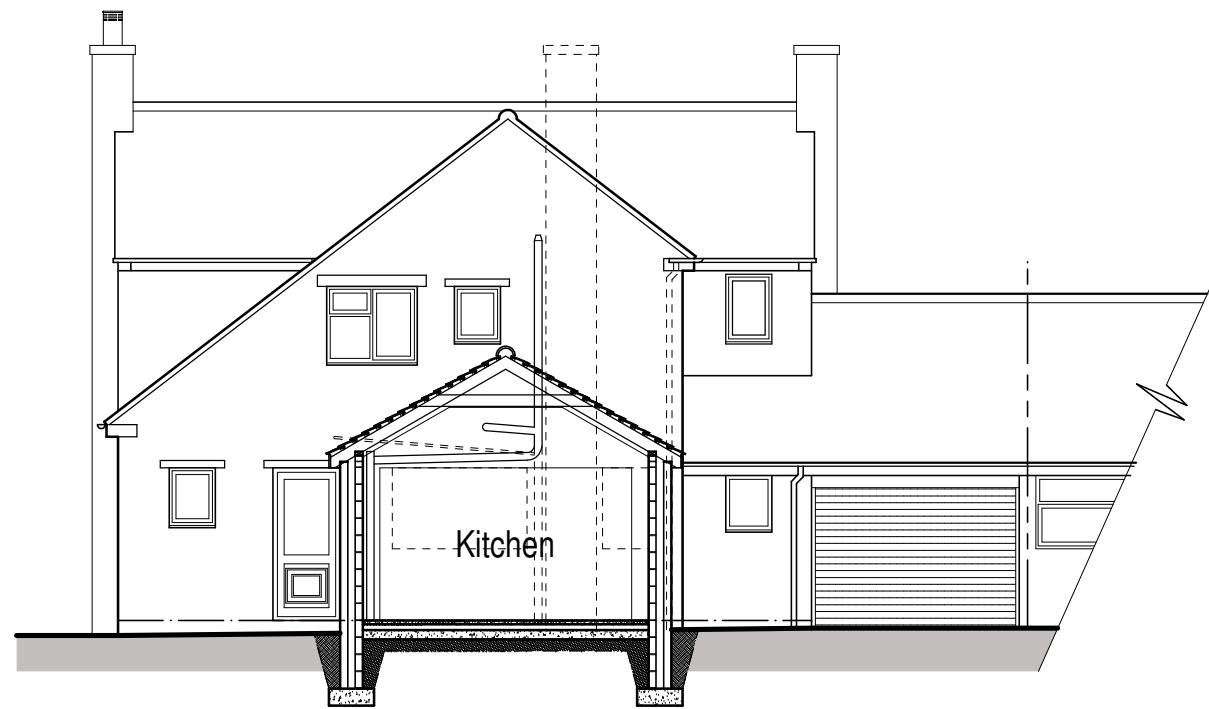
Cross Section
